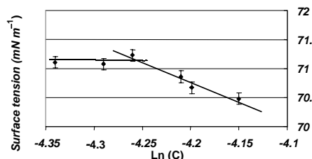
Figure 3. Surface tension isotherm of lead nitrate dissolved in a 0.9 c_0 benzene solution in water, at 25°C. Letter c is c_{\text{Pb}(\text{NO}_3)_2} .
