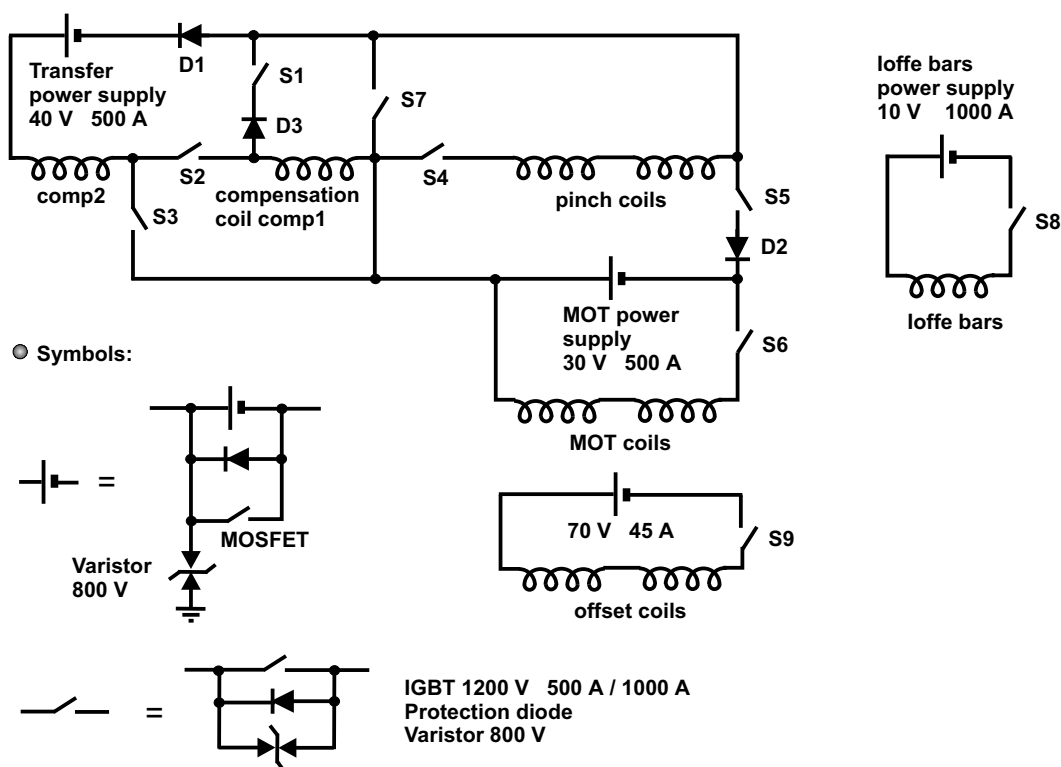
Figure 2.9: The electric circuit used for the magnetic trap. The power supplies deliver up to 1000 A to the field coils. Different configurations can be achieved using IGBT switches, thus enabling the magnetic transfer of the atoms from the MOT to the appendage region, the reuse of the transfer coils as compensation coils and the use of the pinch or the compensation coils to produce the field necessary for Feshbach resonances. The circuit is explained in detail in the text.
