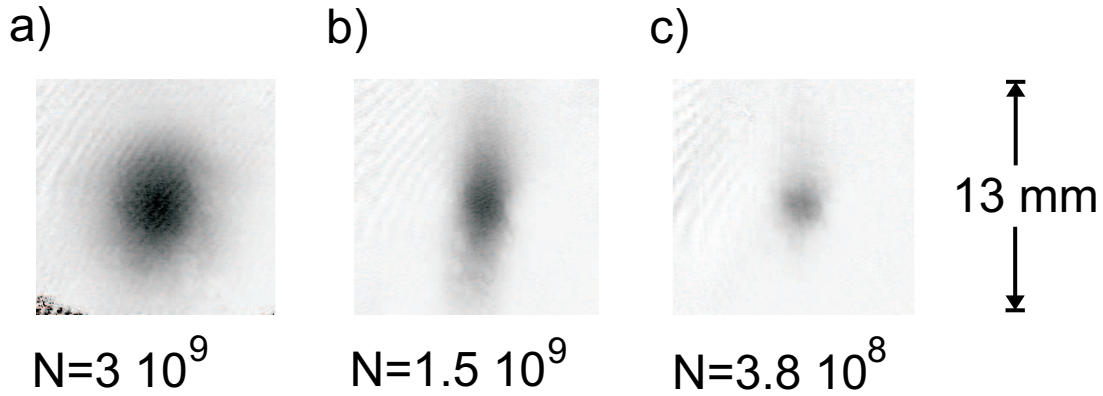
Figure 3.4: Loss of atoms during the transfer to the appendage. a) 3 \times 10^9 atoms after capture in the lower quadrupole trap. b) 1.5 \times 10^9 atoms are left after half of the transfer to the appendage and a reversed transfer to the initial position. The glass cell removes atoms mainly in the horizontal direction, resulting in an elliptic cloud. c) 3.8 \times 10^8 atoms are left after the full transfer and a transfer back to the initial position. Since mainly highly energetic atoms have been removed by collisions with the glass cell, the temperature is decreased by about a factor 3.
