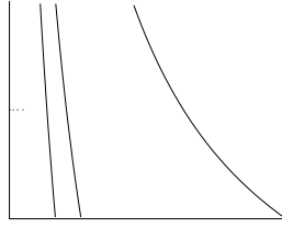
FIGURE 3. The Gauss-map.
