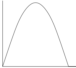
FIGURE 4. T(x) = 4x(1-x) .
