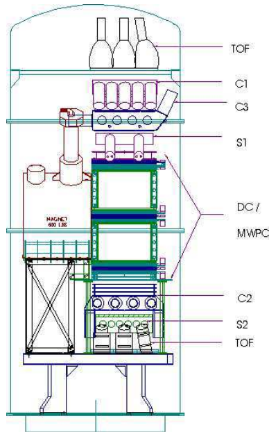
Figure 4.5: Schematic drawing of the IMAX instrument [?]. IMAX has a useful geometry factor of 140 \text{ cm}^2 \text{ sr} . As its basis, IMAX uses the NASA/NMSU Balloon-Borne Magnet Facility payload, with additional detectors and electronics supplied by the collaboration. See text for the abbreviations of all devices.
