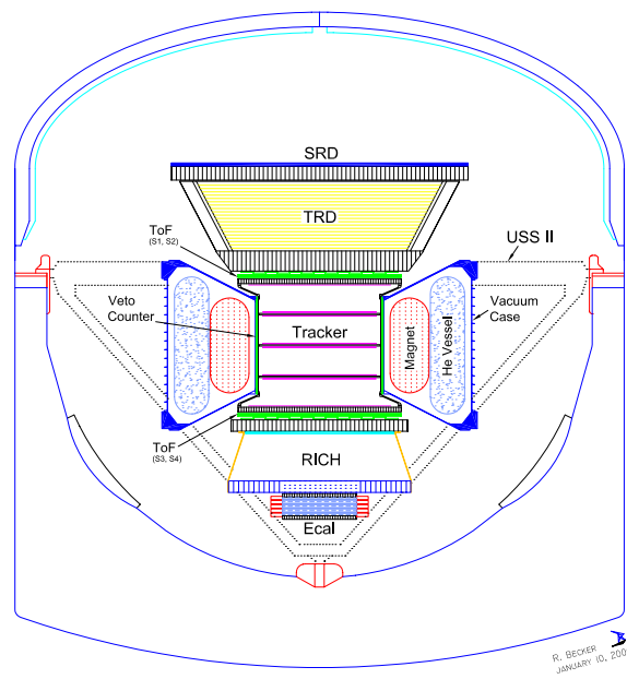
Figure 4.10: AMS02 configuration. Picture is from the AMS Collaboration.
