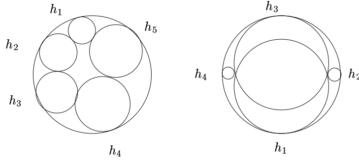
FIG. I.6 – Exemples de bracelets.
