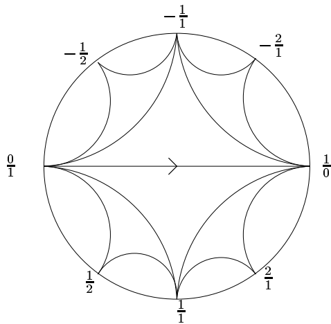
FIG. I.8 – Tessellation de Farey.
