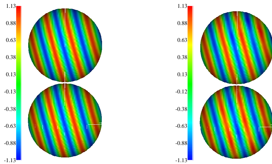
a) \mathcal{C}(\text{IE}+\text{FMM})
