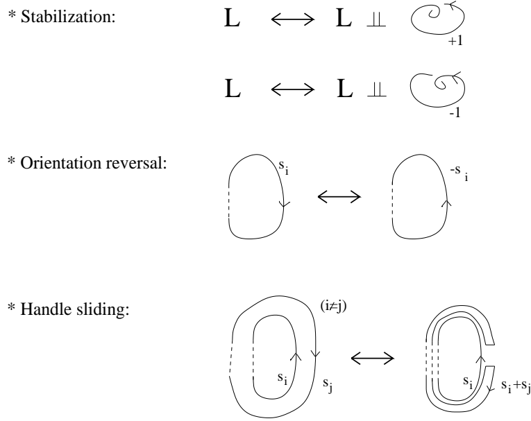
Figure 3.2: Spin^c Kirby's moves
