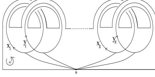
Figure 3.1: The based curves (x_i, y_i)_{i=1}^g on \Sigma_{g,1}
