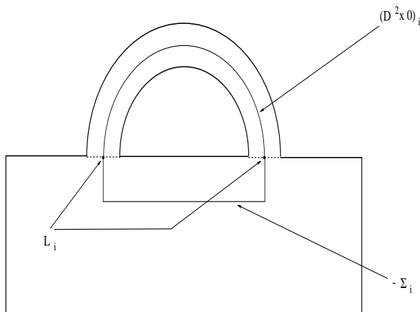
Figure 3.1: The preferred basis of H_2(W_L) .
