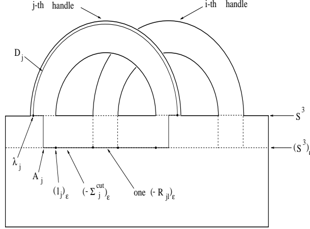
Figure 4.2: A decomposition of the surface S_j
