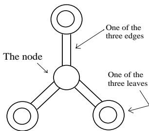
Figure 2.3: A Y -graph.
