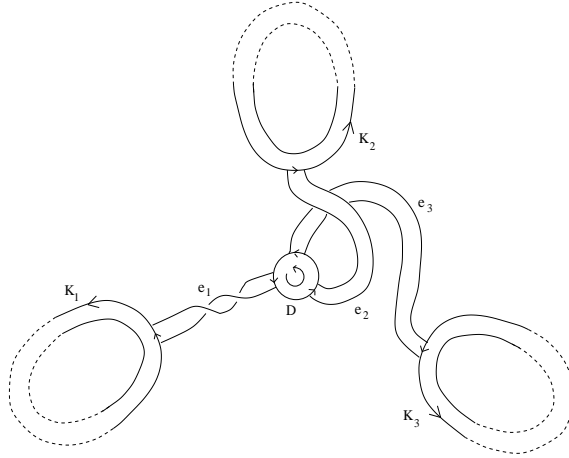
Figure 2.1: Embedding the Y -graph
