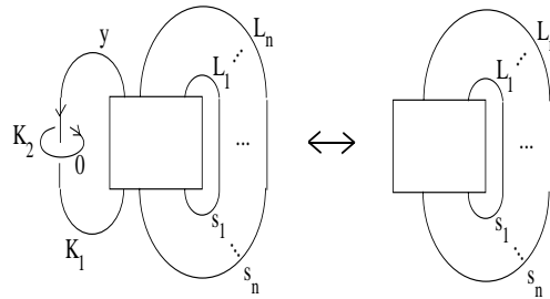
Figure 3.3: A Spin^c -version of the slam dunk move.
