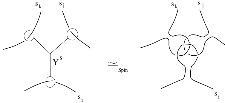
Figure 3.2: A simple Y^s -surgery.
