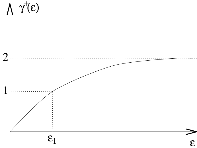
Figure 2: \gamma^+(\epsilon) : mean number of electrons re-emitted by the wall for one incident electron
