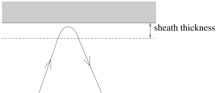
Figure 3: trajectory of an electron of energy \epsilon < \epsilon_s
