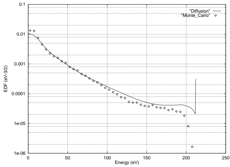
Figure 6: Comparison at z = 3, 4 \text{ cm} from the anode
