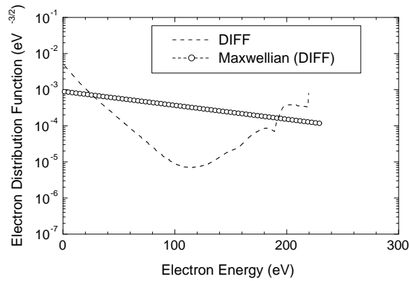
Figure 17: Presence of a beam of electrons of high energy (EEDF at z = 3.4 \text{ cm} ). At this point, the tail of the distribution is very important and the distribution is clearly not Maxwellian.
