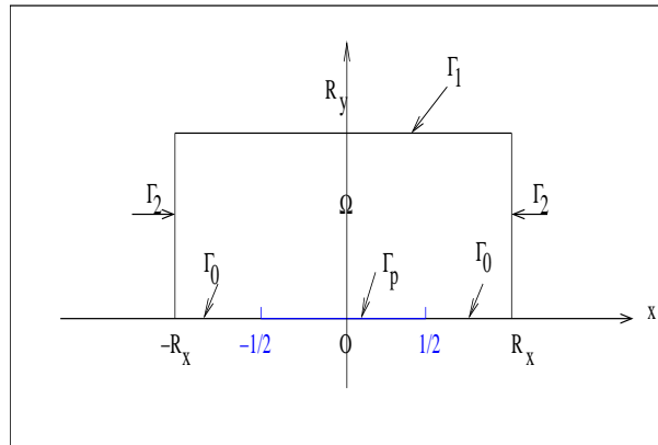
Fig. 1 Study domain
