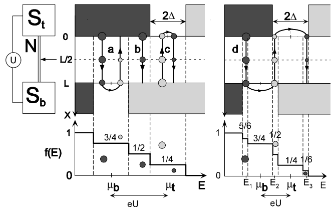
FIG. 1: Left: layout of the experiment: a voltage U is applied between two superconductors ( S ) connected through a normal wire ( N ) of length L . A superconducting probe electrode, figured with an arrow, forms a tunnel junction with the central part of the wire. Top center and top right: representation in the energy (horizontal axis) and position (vertical axis) space of the quasiparticle paths responsible for the current through the normal wire. The excitation spectrum of the top and bottom superconductors has a gap 2\Delta centered on their electrochemical potentials \mu_t and \mu_b ( \mu_t - \mu_b = eU ), with quasielectron states occupied at negative energies (dark areas) and empty (light gray areas) at positive energies. Quasiparticle paths consist of quasielectron (dark disks) and quasihole (light gray disks) trajectories at symmetric energies about \mu_t or \mu_b , connected by Andreev reflection. The area of the disks is proportional to the occupation factor of the quasiparticle state, which varies linearly along the path from 1 to 0. The bottom plots are the energy distribution functions at the center of the wire, at eU > 2\Delta (center) and \Delta < eU < 2\Delta (right).
