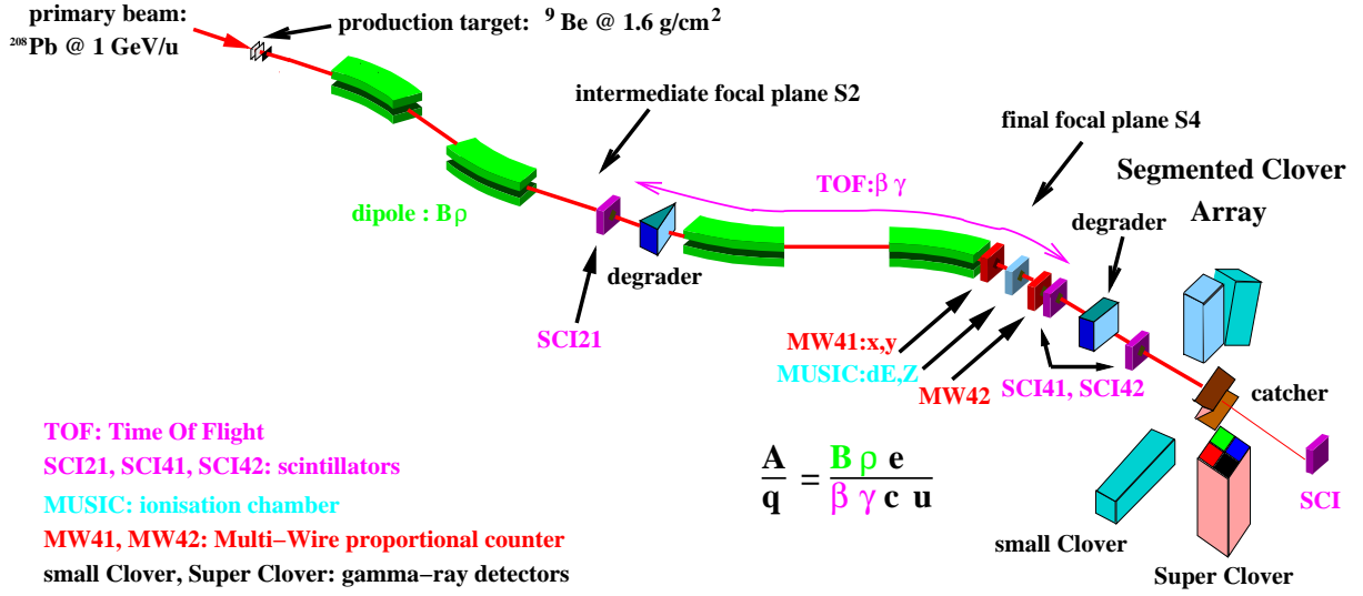
Figure 2.4: The FRagment Separator used to separate and identify the ions produced by projectile fragmentation at GSI coupled with the \gamma detector array.
