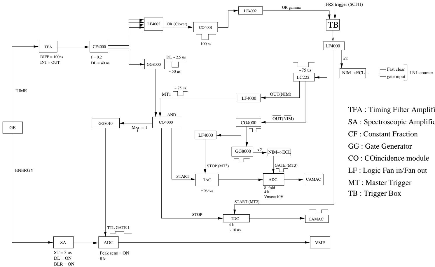
Figure 2.10: Electronics scheme of the \gamma -ray acquisition
