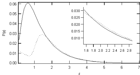
FIG. 7: Distribution function P(\varepsilon) when no shear is applied (stray line) and when a strain square pulse ( \gamma_0 = 0 ) is applied. The inset is a zoom on the region where the overaging is visible.
