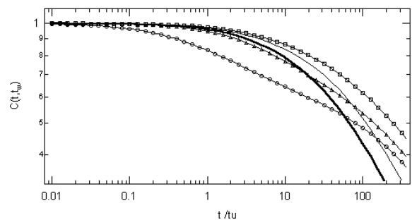
FIG. 9: Same curve that fig5 but for the calculated C(t_w, t + t_w) for t_w = 0.01 tu ( \circ ), 6 tu ( \Delta ), 50 tu ( \square ). The amplitude of the strain is \gamma_0 = 2.5 .
