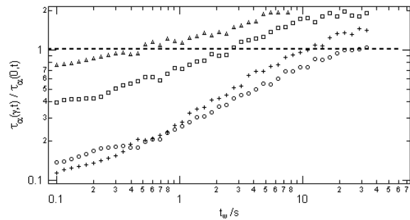
FIG. 6: Normalized \alpha relaxation time for \gamma_0 = 7.9\% at various frequencies: 0.1Hz(o), 1Hz(+), 5Hz ( \square ), 10Hz ( \Delta ). Notice that the importance of the overaging regime increases with the frequency.
