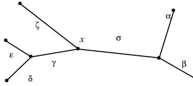
Figure 2.2: \delta_{x,\sigma}(\Delta) = \sigma\alpha^2\beta^2\sigma\gamma\delta^2\epsilon^2\gamma\zeta^2 .
