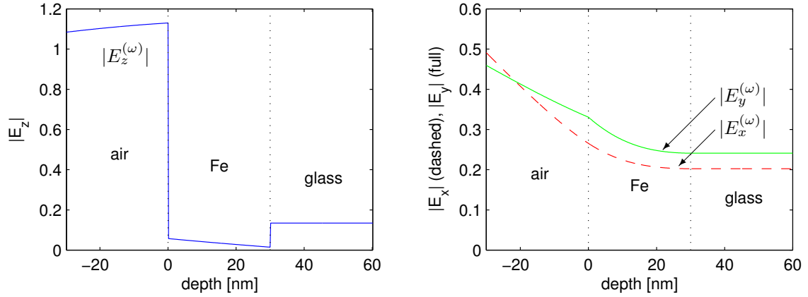
Figure 8.7: In-depth profile of the amplitude of the electric field components |E_x| (incident unitary s wave), |E_y| , |E_z| (incident unitary p wave) for an air/Fe(30 nm)/glass structure, at E = 1.55 eV, at a fixed incidence angle \varphi = 45^\circ . \Im(\varepsilon_{0,Fe}^{(\omega)}) is assumed to be non-zero (Appendix 8.11).
