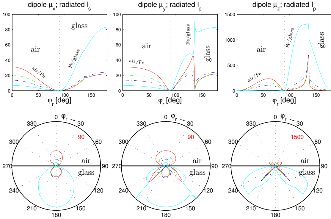
Figure 8.8: Angular dependence of radiated intensity of the s and p polarized light, I_s , I_p , emitted by unitary dipoles \mu^{(2\omega)} oriented in the x , y and z directions in the air/Fe(30 nm)/glass structure. The radiating dipoles are assumed to be located on the air/Fe interface (red full line), on the Fe/glass interface (bright blue full line) and 5 and 10 nm below the top air/Fe interface (green and blue dashed lines). \Im(\varepsilon_{0,Fe}^{(2\omega)}) is assumed to be non-zero (Appendix 8.11).
