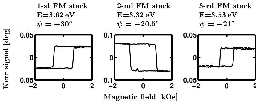
Figure 5.18: Individual PMOKE hysteresis loops of each TbFe stack in the (\text{TbFe}/\text{Si}_3\text{N}_4)_4 system, obtained when choosing E and \psi to cancel Kerr signals of two TbFe stacks. Values of E , \psi are indicated above each loop.
