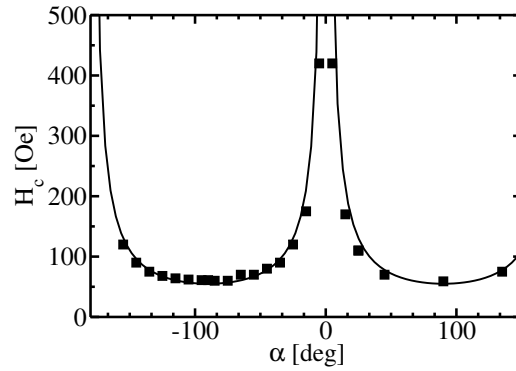
Figure 6.7: Variation of the in-plane coercive field with the sample rotation angle \alpha . The origin \alpha = 0 corresponds to \mathbf{H} \parallel \hat{X} . The full line shows a fit of the data by the H_c = H_{c0}/|\sin \alpha| function, with H_{c0} = 55 Oe.
