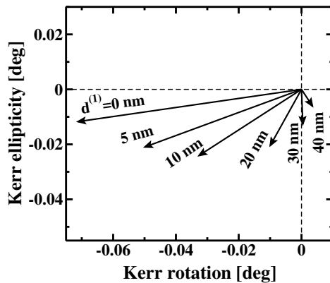
Figure 5.1: Variation of the Kerr vector with increasing the overlayer thickness d^{(1)} for the \text{Au}(d^{(1)})/\text{Co}(1\text{ nm})/\text{Au} system, calculated for \varphi = 0^\circ , E = 3\text{ eV} .
