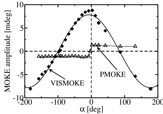
Figure 6.6: Dependence of the s-MOKE ellipticity amplitudes of both square loop ( \Delta ) and S-shape ( \blacklozenge ) MOKE contributions on sample rotation \alpha , as determined from hysteresis loops presented on Figure 6.4. The S-shape contribution is fitted by a cosine function.
