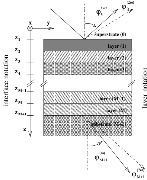
Figure A.1: Definition of the Cartesian referentials for the sample ( \hat{x} , \hat{y} , \hat{z} ) and the incidence ( \hat{s}_+ , \hat{p}_+ , \hat{k}_+ ) and the reflected (or radiated) ( \hat{s}_- , \hat{p}_- , \hat{k}_- ) light referentials.
