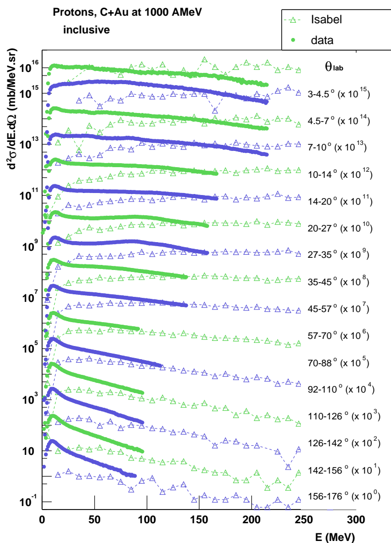
Figure 5.15: The proton kinetic energy spectra (full circles) for C+Au at 1000 AMeV are compared to the Isabel cascade model (open triangles) at 3^\circ \leq \theta_{lab} \leq 176^\circ for inclusive data.
