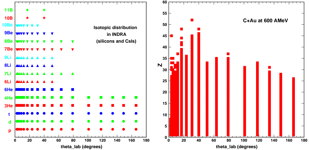
Figure 3.4: Isotopic (left panel) and charge (right panel) distributions in the INDRA detector as function of the polar angle \theta_{lab} for the reaction C+Au at 600 AMeV.
