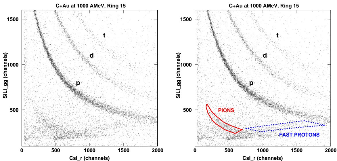
Figure 7.3: Matrix SiLi versus Csl for the reaction C+Au at 1000 AMeV, for the ring 15 ( 126^\circ \leq \theta_{lab} \leq 142^\circ ). In the left panel, the three main lines correspond to the protons, deuterons and tritons stopped in the Csl crystal. In the right panel, the area surrounded by a solid line corresponds to the \pi^+ 's stopped in the Csl. The dashed line indicates the fast protons ( E_k \geq 150 MeV) punching through the Csl.
