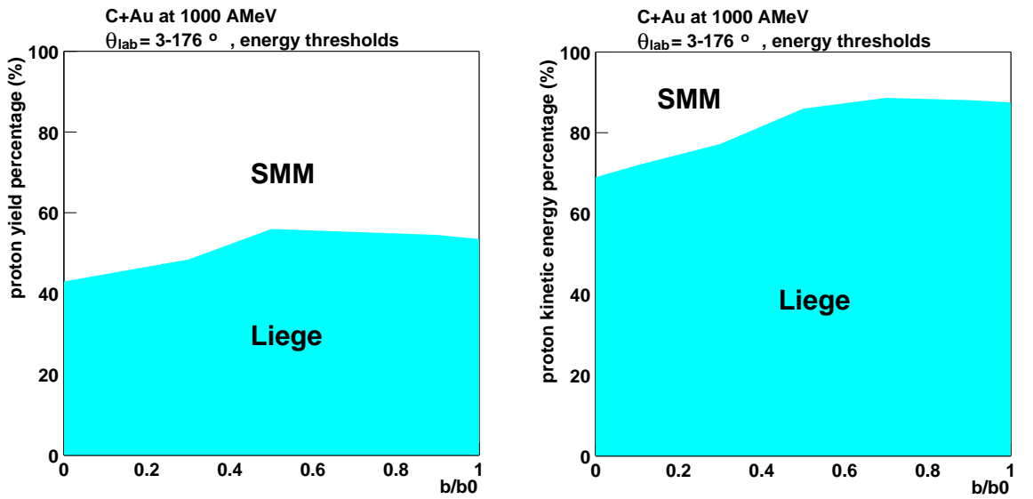
Figure 5.18: Proportions of proton yields (left panel) and kinetic energy (right panel) between cascade (Liège) and multifragmentation (SMM) for the system C+Au at 1000 AMeV with the angular coverage ( 3^\circ \leq \theta_{lab} \leq 176^\circ ) and the energy threshold conditions of the INDRA detector.
