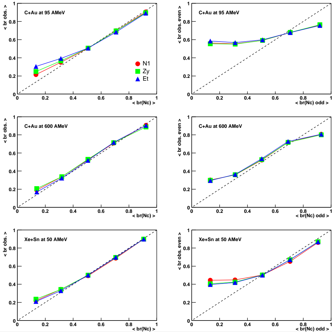
Figure 4.12: Left panels: mean measured impact parameter for all modules ( \langle b_r(ops) \rangle ) as a function of gates in impact parameter b_r(N_C) for all modules ( \langle b_r(cut) \rangle ). Right panels: mean measured impact parameter for even modules ( \langle b_r(ops, even) \rangle ) as a function of gates in impact parameter b_r(N_C) for odd modules ( \langle b_r(cut) \rangle ). The diagonal lines correspond to the perfect correlation.
