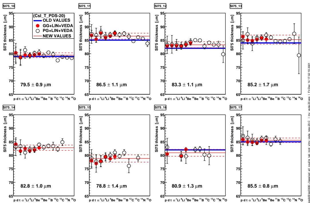
Figure 3.11: Thickness of the silicon Si75 for each ring, determined from \alpha source runs. One compares in these panels the thickness values measured in previous campaigns when they exist (thick full lines), the new values (thin full lines), and the values used to calculate the new values coming from low (PG, empty circles) and high (GG, full circles) gain with the use of VEDA energy loss tables. The thickness values are indicated in each panel [Luk02].
