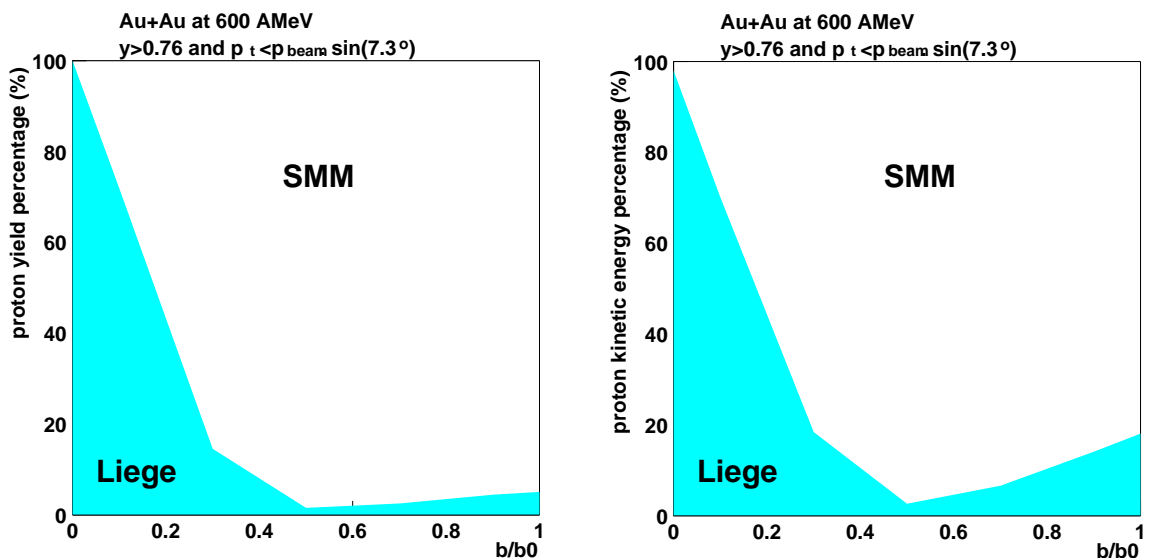
Figure 5.20: Proportions of proton yields (left panel) and kinetic energy (right panel) between cascade (Liège) and multifragmentation (SMM) for the system Au+Au at 600 AMeV with the momentum ( p_t < p_{beam} \cdot \sin(7.3^\circ) ) and rapidity ( y > 0.76 ) conditions applied in ALADIN analysis.
