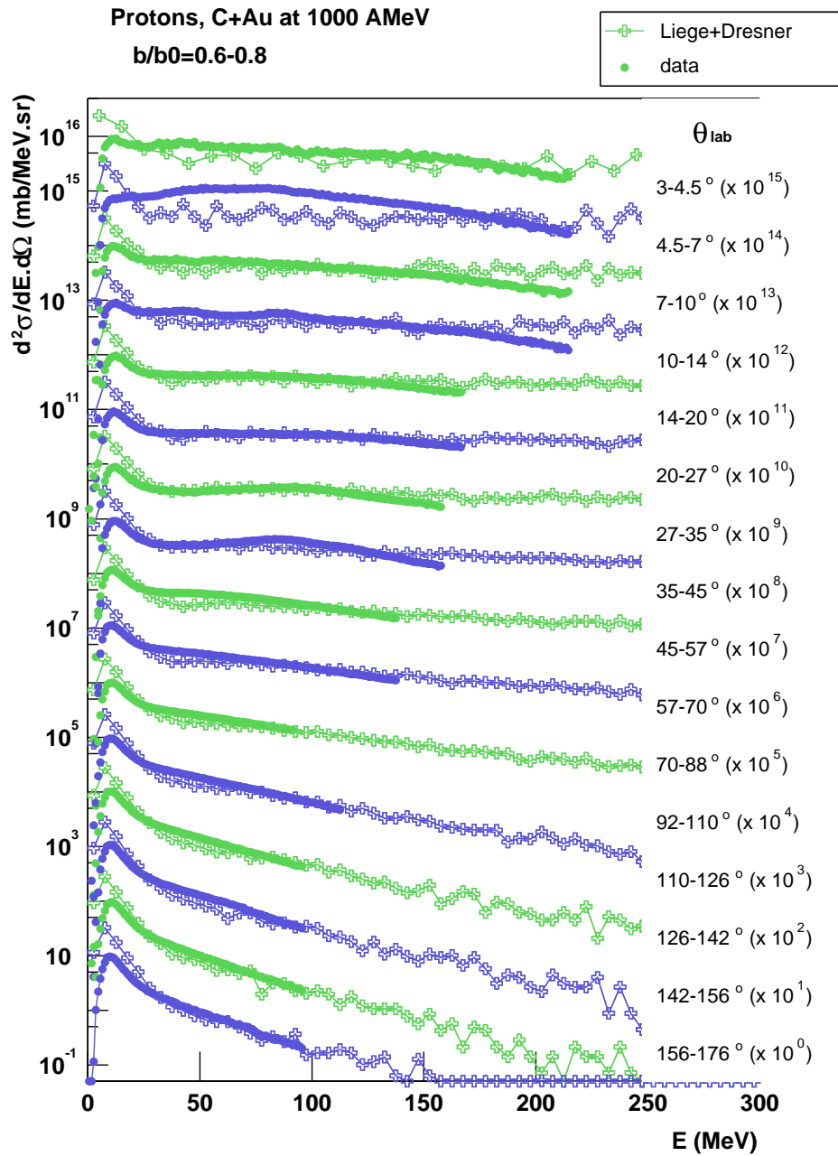
Figure D.4: The proton kinetic energy spectra for C+Au at 1000 AMeV are compared to the Liège cascade model (high energies) coupled to the evaporation Dresner code (low energies) for b/b_0=0.6-0.8 (almost peripheral collisions).
