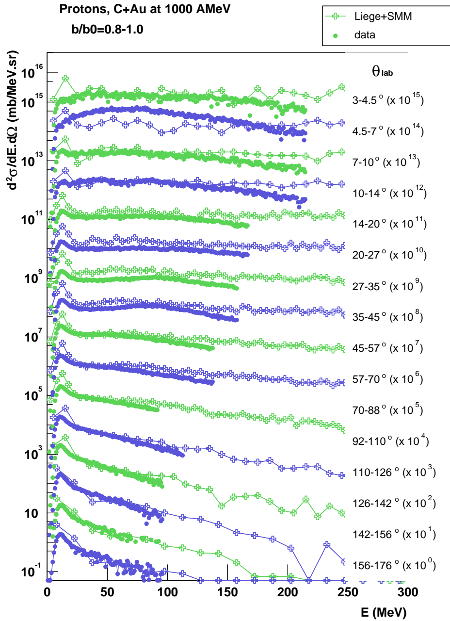
Figure D.10: The proton kinetic energy spectra for C+Au at 1000 AMeV are compared to the Liège cascade model (high energies) coupled to SMM (low energies) for b/b_0=0.8-1.0 (peripheral collisions).
