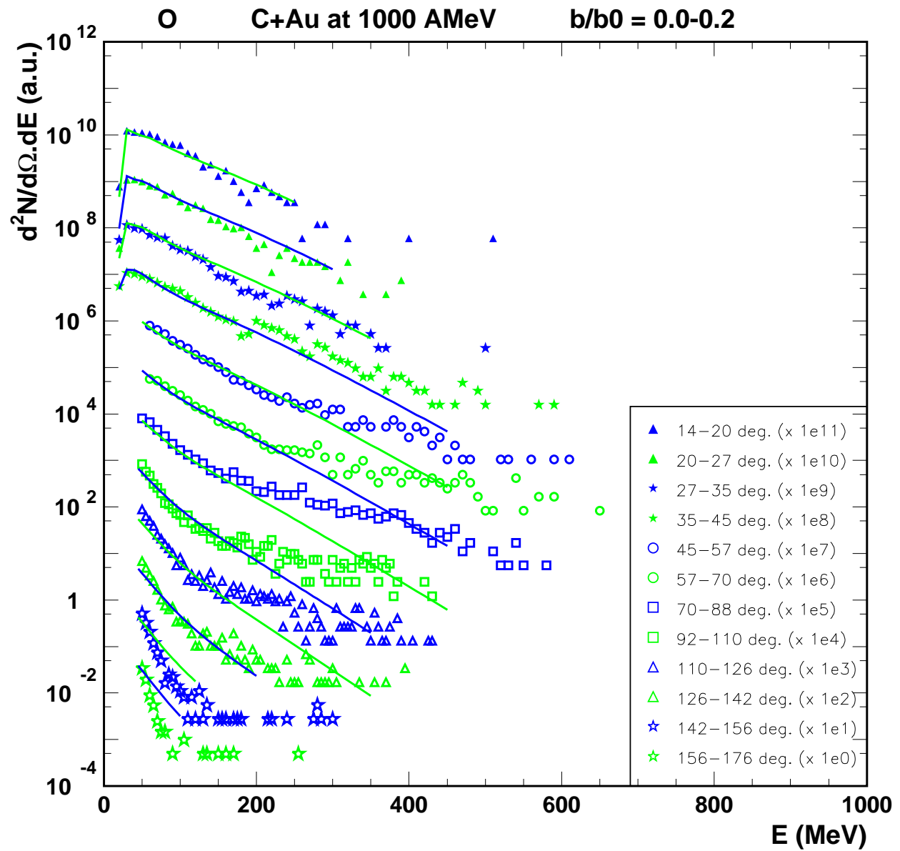
Figure 6.9: Global fit (full lines) of oxygen kinetic energy spectra (symbols) for the system C+Au at 1000 AMeV for central collisions ( b/b_0=0.0-0.2 ) at 14 \leq \theta_{lab} \leq 176^\circ .
