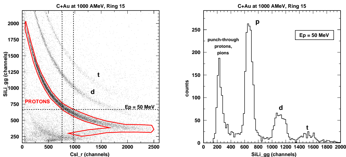
Figure 5.1: Left panel: matrix SiLi\_gg (high gain) versus CsLr (fast component) for the ring 15 ( 126^\circ \leq \theta_{lab} \leq 142^\circ ) for the reaction C+Au at the incident energy of 1000 AMeV. One can observe, from top to bottom, curved lines corresponding to the tritons (t), the deuterons (d), and the protons. Protons are identified by a gate drawn around the stopped and punch-through proton line. Right panel: projection of the channel range in CsLr (vertical dashed lines in the left panel) corresponding to the proton kinetic energy E_p = 50 \pm 3 MeV in SiLi\_gg (horizontal dashed line in the left panel).
