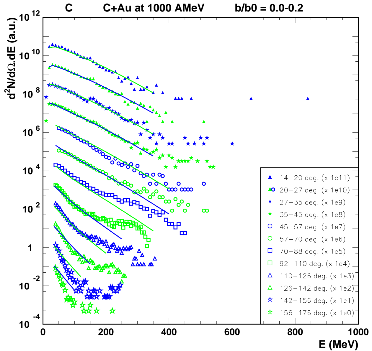
Figure 6.7: Global fit (full lines) of carbon kinetic energy spectra (symbols) for the system C+Au at 1000 AMeV for central collisions ( b/b_0=0.0-0.2 ) at 14 \leq \theta_{lab} \leq 176^\circ .
