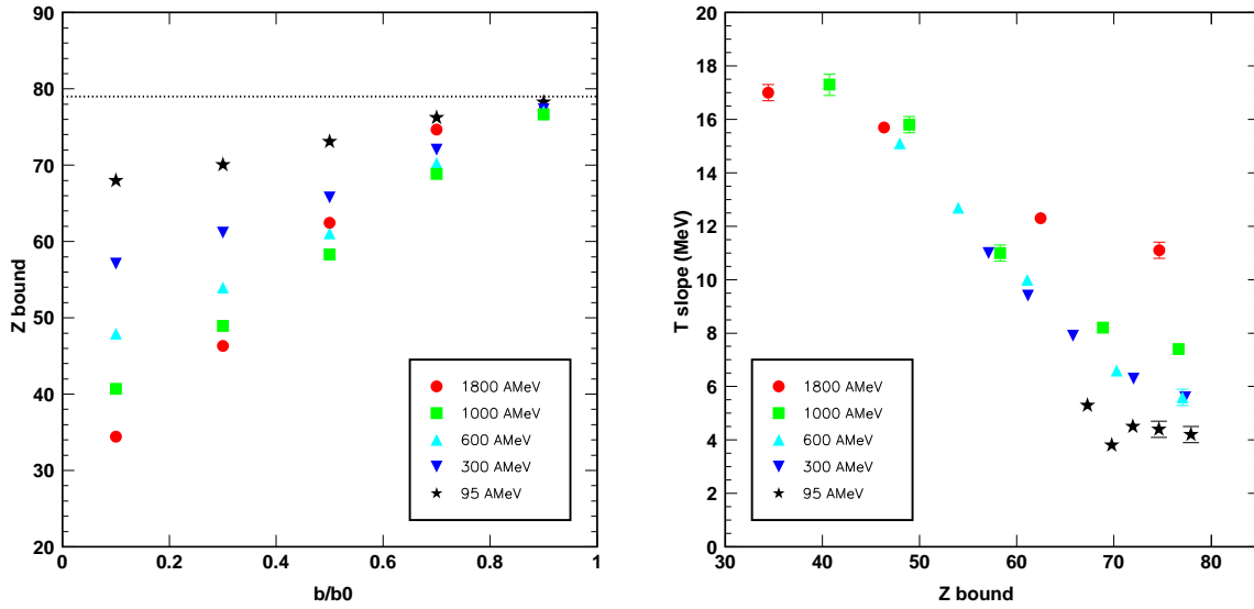
Figure 6.11: Left panel: Z_{bound} ( Z_{Au} - M_{hydrogen} ) at 45 \leq \theta_{lab} \leq 142^\circ and normalised over 4\pi as a function of the reduced impact parameter b/b_0 for the system C+Au at the incident energies from 95 to 1800 AMeV. Right panel: Carbon slope temperature of the target source as a function of Z_{bound} for the system C+Au at the incident energies from 95 to 1800 AMeV.
