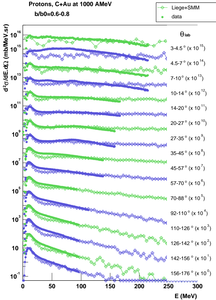
Figure D.9: The proton kinetic energy spectra for C+Au at 1000 AMeV are compared to the Liège cascade model (high energies) coupled to SMM (low energies) for b/b_0=0.6-0.8 (almost peripheral collisions).
