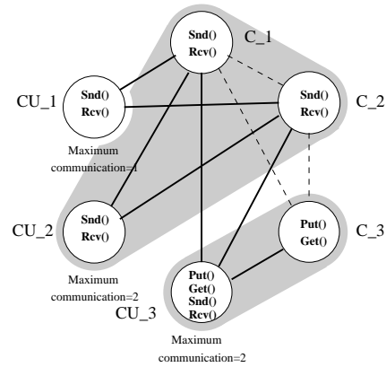
4.16.2: Solution d'allocation
