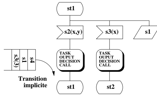
3.12.2: Transition implicite
