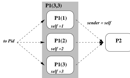
FIG. 3.9: Instances multiples de processus SDL
