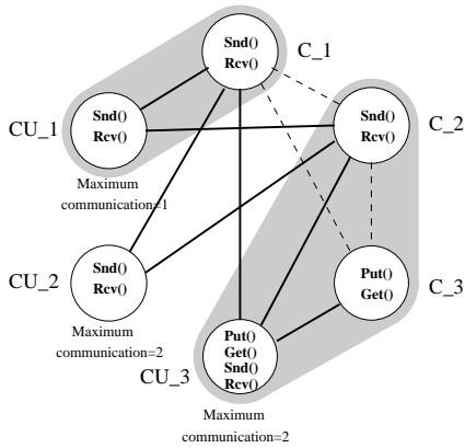
4.16.1: Solution d'allocation
