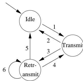
FIG. 6.5: Automate de l'état Established
