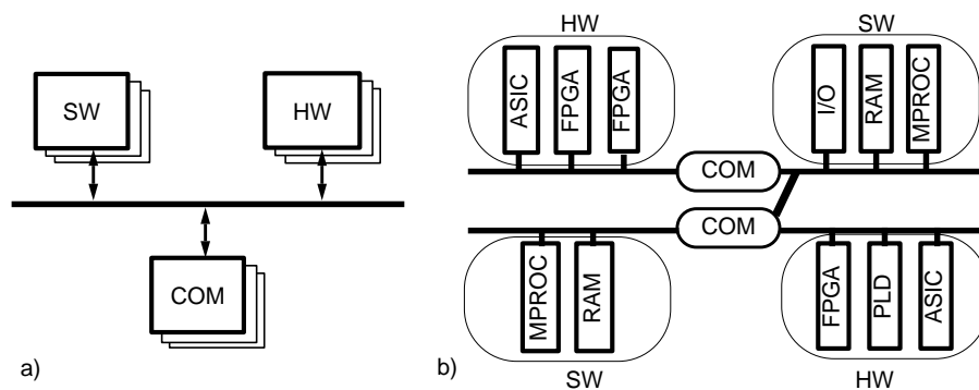
figure 5.4 : Architectural Model: a) architectural model. b) Hardware/software platform.
