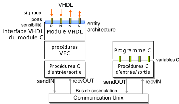
figure 3.10: Interface VHDL-C
