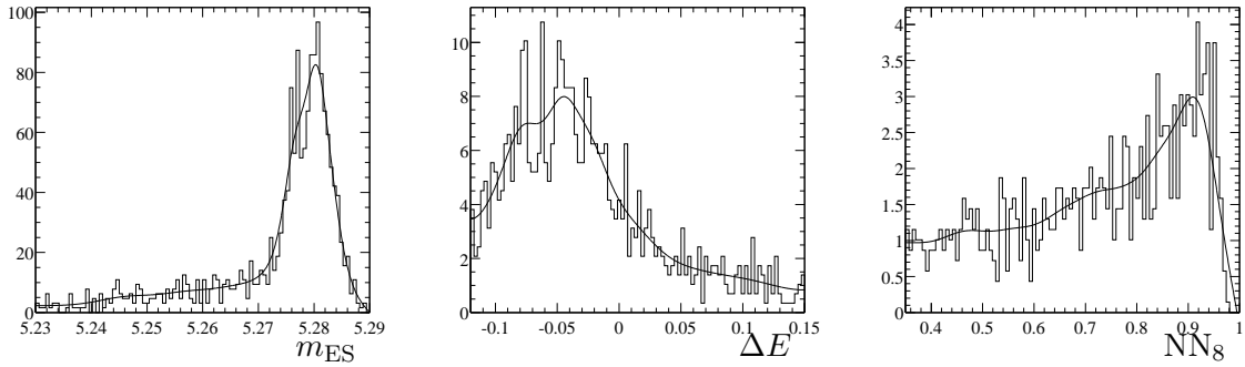
(c) B^0 \rightarrow (K^{**} \pi)^0
