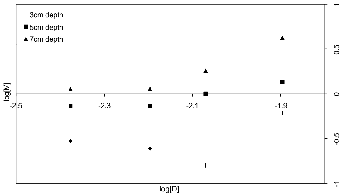
Figure 3.7 Log - Log dependency between the overturning moment (M) and the model diameter (D). Results for tap root models with four different diameters (D 1 =4.2 mm, D 2 =6.35 mm, D 3 =8.50 mm, D 4 =12.70 mm) embedded at three different depths (3 cm, 5 cm, and 7 cm) in agricultural soil.
