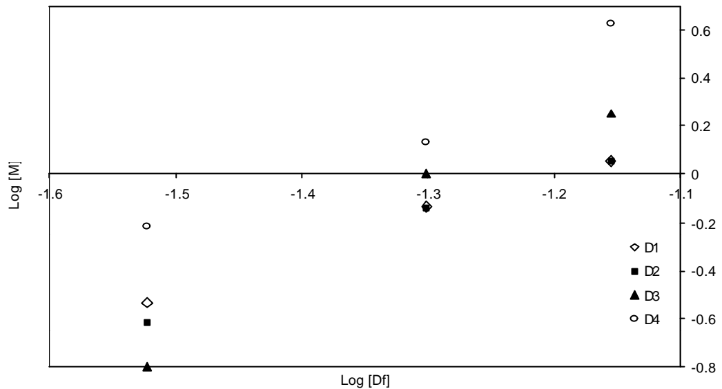
Figure 3.6 Log-Log dependency between the overturning moment (M) and the embedment depth (D f ). Results for the tap root models of four different sizes (D 1 =4.2 mm, D 2 =6.35 mm, D 3 =8.50 mm, D 4 =12.70 mm) embedded at three different depths (3 cm, 5 cm, and 7 cm) in agricultural soil.
