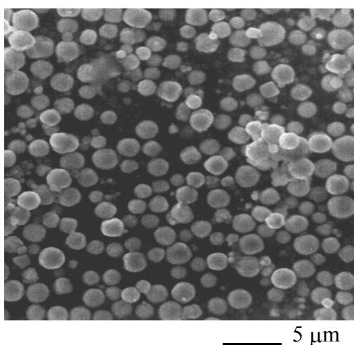
Fig. 1 : Scanning Electron Microscopy (SEM) picture of copper powder. Particles have an average diameter of 1.05 \mu\text{m} with a standard deviation of 0.26.
