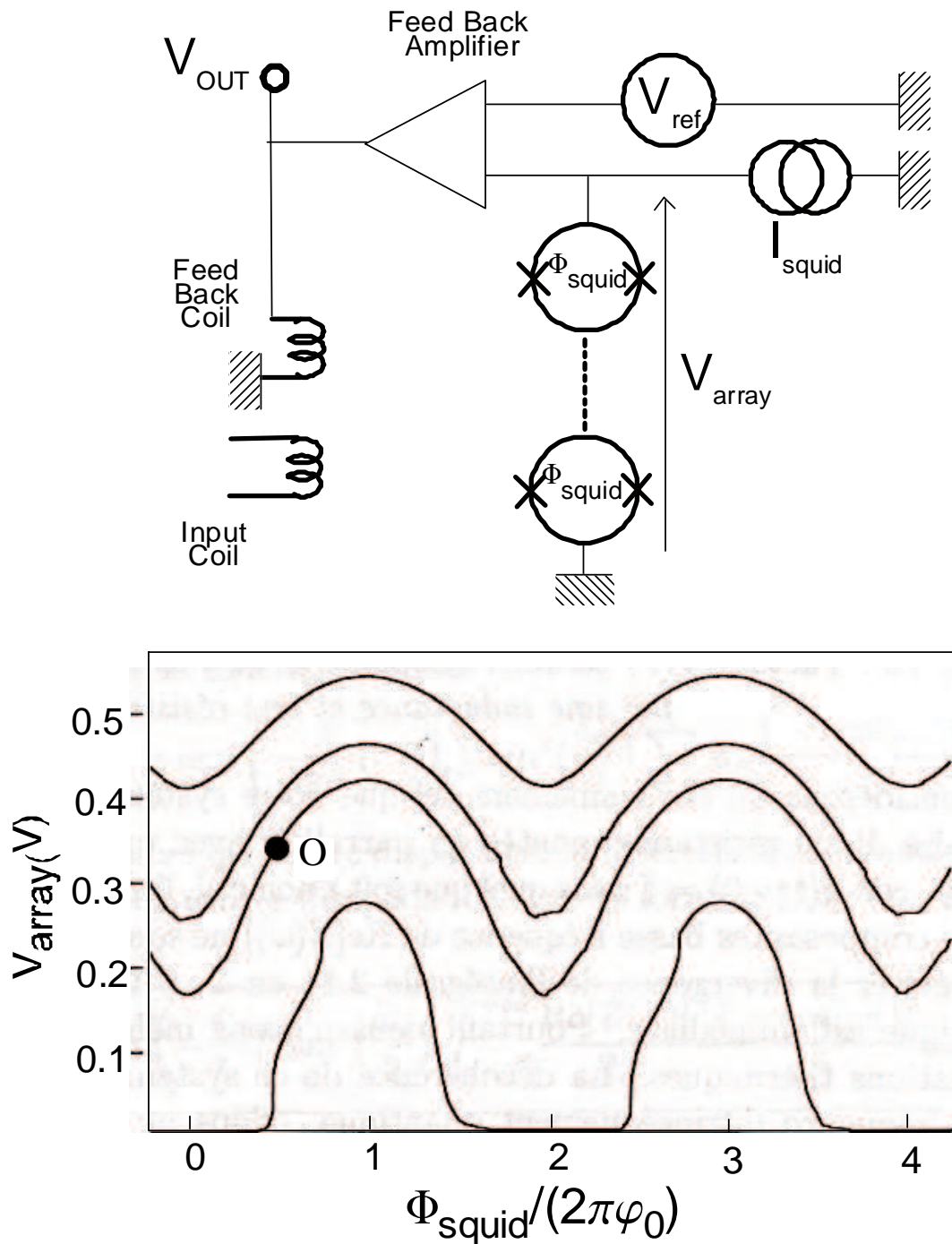
Figure 2.22: Top panel: Scheme of the feed-back loop in which the array of DC SQUIDS is embedded. The series of SQUIDS is biased by a current I_{\text{squid}} . The voltage V_{\text{array}} across the array, which depends on the flux \Phi_{\text{squid}} through the squids, is measured using an amplifier. In the feed-back mode, this voltage is maintained at a fixed value V_{\text{ref}} . Bottom panel: Measured V_{\text{array}}-\Phi_{\text{squid}} characteristic for 4 different values of I_{\text{squid}} . The irregularities in the characteristic are due to mutual inductance phenomena between the SQUIDS. The feed-back amplifier gain is tuned so that the flux sent by the feed-back coil maintains the SQUID array at a constant working point like O. The output of the measurement is the output signal of the feed-back amplifier.
