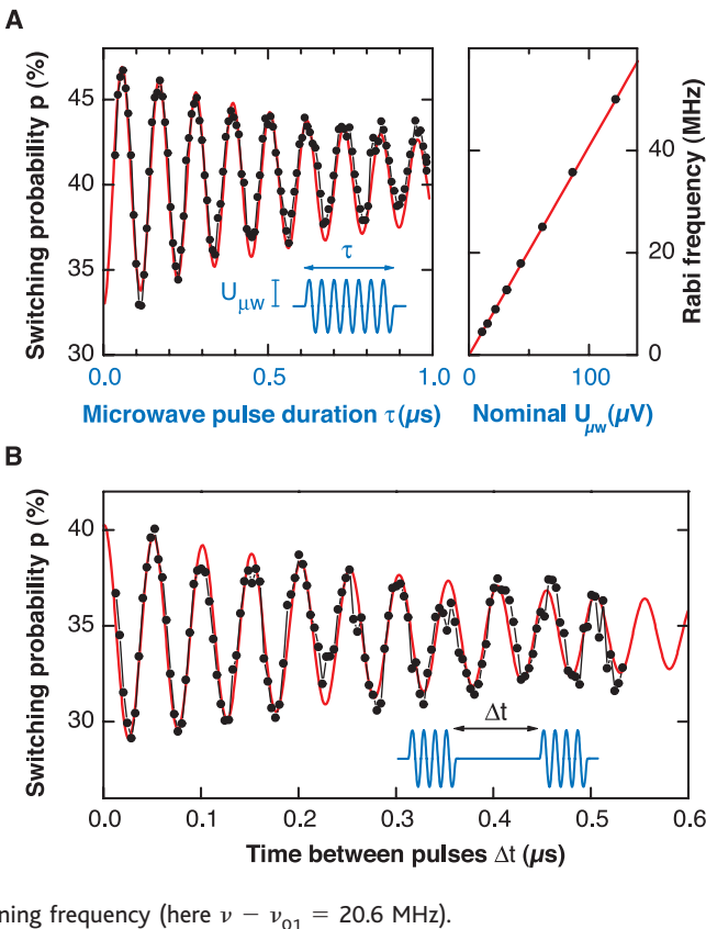
Fig. 3. (A) Left: Rabi oscillations of the switching probability p ( 5 \times 10^4 events) measured just after a resonant microwave pulse of duration \tau . Data were taken at 15 mK for a nominal pulse amplitude U_{\mu w} = 22 \mu V (joined dots). The Rabi frequency is extracted from an exponentially damped sinusoidal fit (continuous line). Right: Measured Rabi frequency (dots) varies linearly with U_{\mu w} as expected. (B) Ramsey fringes of the switching probability p ( 5 \times 10^4 events) after two phase-coherent microwave pulses separated by \Delta t . Joined dots: Data at 15 mK; the total acquisition time was 5 mn. Continuous line: Fit by exponentially damped sinusoid with time constant T_\phi = 0.50 \mu s. The oscillation corresponds to the beating of the free evolution of the spin with the external microwave field. Its period indeed coincides with the inverse of the detuning frequency (here \nu - \nu_{01} = 20.6 MHz).
