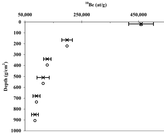
Figure 33: In situ-produced 10 Be concentrations as a function of depth along the Itaberaba massive quartz vein. Crosses correspond to the experimental data. Open circles represent the theoretical depths calculated for the measured 10 Be assuming a mean erosion rate of 9.0 \pm 0.5 m.My -1 (deduced from the surficial sample BR96-12F) and using a 5 at/g/year 10 Be production rate.
