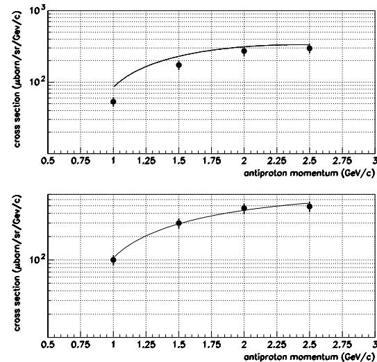
FIG. 2.— Here are displayed the antiproton production cross section in p+C (top) and p+Al (bottom) collisions at 12 GeV laboratory kinetic energy. Filled circles are experimental data Sugaya et al. 1998 and the lines are from our DTUNUC simulations. The error bars have been assumed to be 15%. This value is usual for such experiments and was suggested by a \chi^2 analysis combining most data available.
