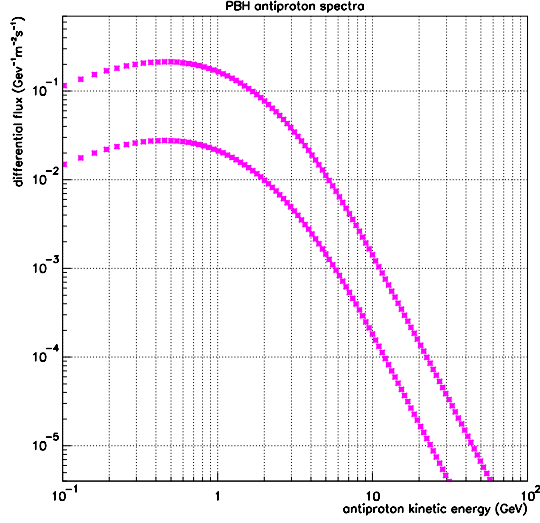
Fig. 5. TOA primary antiproton flux with the standard mass spectrum after propagation for \rho_{\odot}^{\text{PBH}} = 10^{-32} \text{ g cm}^{-3} and extreme astrophysical models.
