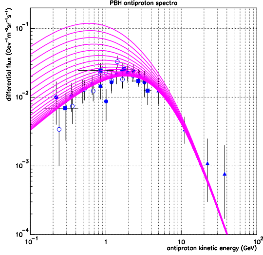
Fig. 6. Experimental data from BESS95 (filled circles), BESS98 (circles), CAPRICE (triangles) and AMS (squares) superimposed with mean theoretical PBH spectra for \rho_{\odot}^{\text{PBH}} between 5 \times 10^{-35} g cm ^{-3} (lower curve) and 10^{-32} g cm ^{-3} (upper curves).
