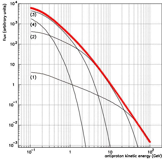
Fig. 1. Primary antiproton flux with the standard mass spectrum before propagation (in arbitrary units). Curve (1) is for M \in [M_{\text{Pl}}, 10^{12} \text{ g}] , curve (2) is for M \in [10^{12} \text{ g}, 10^{13} \text{ g}] , curve (3) is for M \in [10^{13} \text{ g}, 5 \times 10^{13} \text{ g}] , curve (4) is for M > 5 \times 10^{13} \text{ g} and the thick line is the full spectrum.
