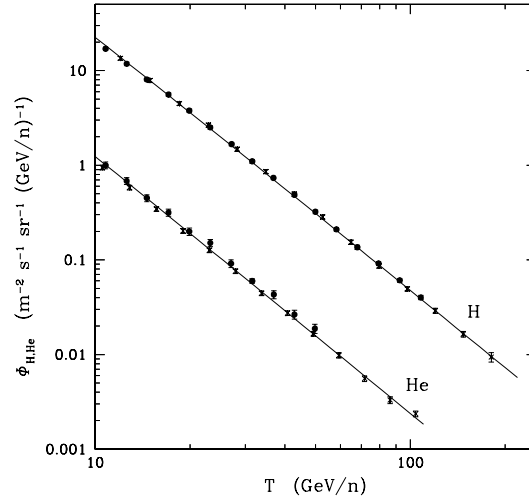
FIG. 1.—Upper (lower) curve displays the measured proton (helium) flux along with an analytical fit (see text). On both curves, data are from AMS (Alcaraz et al. 2000a, 2000b, 2000c; crosses) and BESS (Sanuki et al. 2000; filled circles). [See the electronic edition of the Journal for a color version of this figure.]
