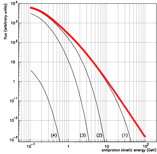
Fig. 2. Primary antiproton flux with the standard mass spectrum before propagation (in arbitrary units) with different reheating temperatures. Curve (1) is for T_{\text{RH}} = 3 \times 10^9 \text{ GeV} , curve (2) is for T_{\text{RH}} = 10^9 \text{ GeV} , curve (3) is for T_{\text{RH}} = 6 \times 10^8 \text{ GeV} , curve (4) is for T_{\text{RH}} = 3 \times 10^8 \text{ GeV} and the thick line is the spectrum without any cutoff.
