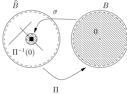
Figure 1.2: Construction of Kato surfaces
