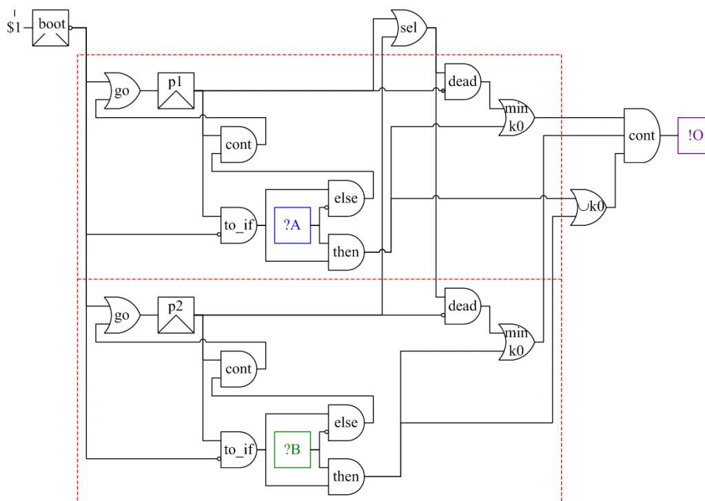
Figure 2.2: Le circuit AB_0
