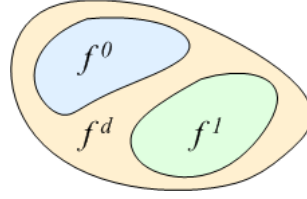
Figure 3.4: Ensembles f^0 , f^1 et f^d = \overline{f^0 + f^1}
