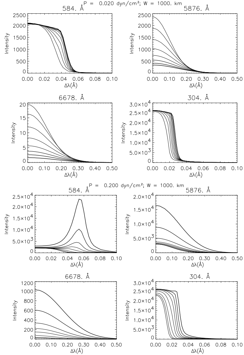
Fig. 8. Half emergent line profiles for one slab width (1000 km) at 0.02 \text{ dyn/cm}^2 (four top panels) and 0.2 \text{ dyn/cm}^2 (four bottom panels). The increase of line thickness corresponds to an increase of temperature. The different temperatures are 6000, 8000, 10000, 12000, 14000, 16000, 18000, and 20000 K. Same units as in Fig. 5.
