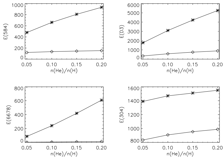
Fig. 15. Integrated intensities (in cgs units) for 4 lines as a function of the abundance computed for 2 models: T = 6000 K, P = 0.02 dyn/cm 2 and W = 1000 km ( \diamond ); T = 18000 K, P = 0.2 dyn/cm 2 and W = 1000 km (*).
