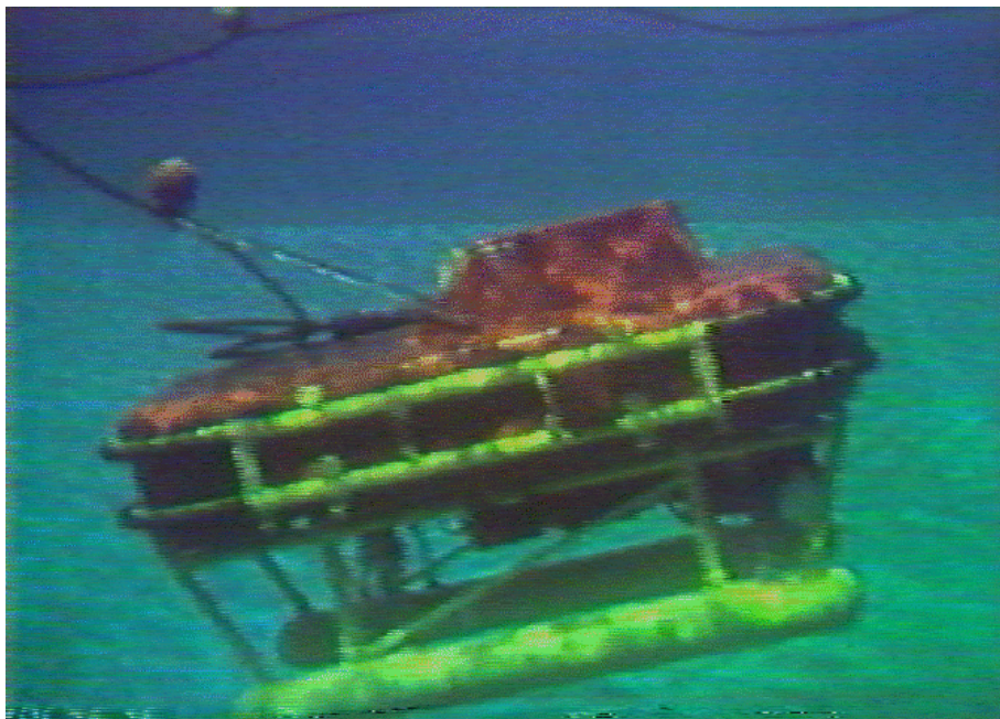
Figure 2.2: ROV ANGUS 002.
