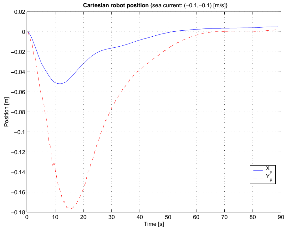
Figure 7.3: Experimental results with sea current \mathbf{V}_c = [-0.1, -0.1]^T : Cartesian robot's position.
