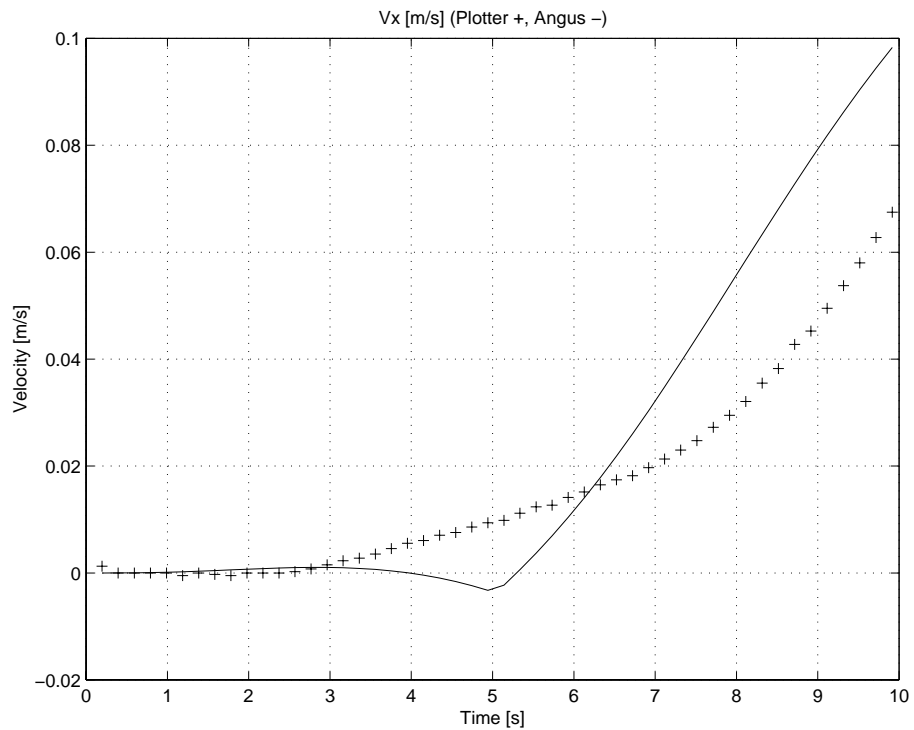
Figure 3.9: Full sway thrusters experiment: surge velocity vs time.
