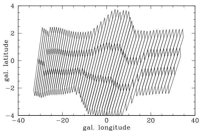
Fig. E-26. Galactic map of the observations for the DENIS “Bulge” project.
