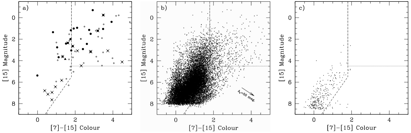
Fig. 5. a) ISOGAL ( [7]-[15] , [15] ) colour-magnitude diagram for the sources associated with BWHZ radio sources and with good detections at both 7\ \mu\text{m} and 15\ \mu\text{m} . Small open circles refer to unclassified radio sources, either non associated with IRAS sources, with low association probability or with ambiguous IRAS colours/fluxes (see BWHZ); filled circles represent UC HII or candidate UC HII; the triangle marks the only PN in the sample. Sources with association distance greater than 8 arcsec are marked with a cross. b) ( [7]-[15] , [15] ) colour-magnitude diagram for all the ISOGAL sources within the BWHZ survey region. c) ( [7]-[15] , [15] ) colour-magnitude diagram for a compilation of ISOGAL fields at high galactic latitude: all fields with |b| \geq 3^\circ , except those in the Magellanic Clouds. In all diagrams the dashed line shows the criteria used to derive YSO candidates in Paper II, the dotted horizontal line shows the more conservative limit on [15] adopted in this paper (see Sect. 5). The extinction vector for A_V = 50\ \text{mag} is shown in panel b) (assuming the extinction law provided by Jiang et al., private communication).
