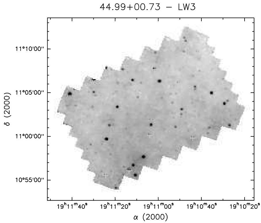
Fig. 4. Field A (44.99+00.73). The 15 μm image with YSOs marked with a cross.
