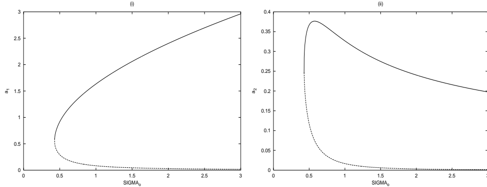
Figure 2.14: Subharmonic frequency-response curves. (i) corresponding for a_1(\sigma_4) and (ii) for a_2(\sigma_4) with the parameters \gamma_{o1} = 0.01 ; \lambda_{o1} = 0.2 ; \lambda_{o2} = 0.4 ; \beta = 0.6 ; \sigma_2 = 2.0 and (a): E = 0.5 , (b) : E = 1.0 .
