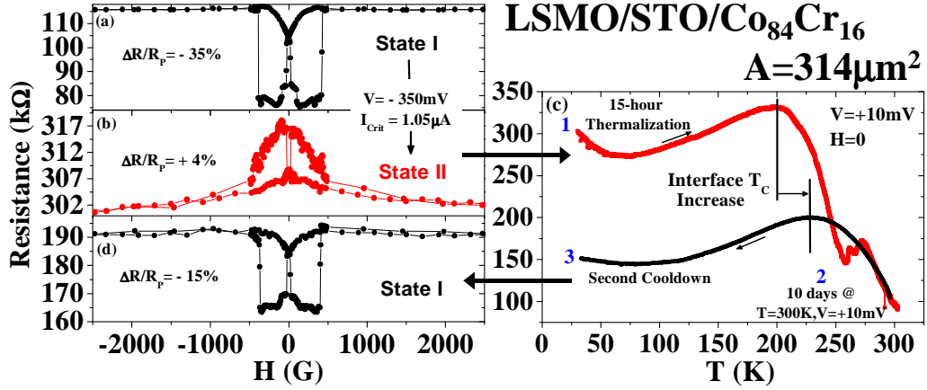
Figure 7.4: Sample B. History of a 314 \mu m^2 LSMO/STO/Co 84 Cr 16 (A11689) junction: R(H) loops at V = +10mV depicting (a) State I and (b) State II. (c) Thermalization to T = 300K and forming at V = +10mV lead to an increase in LSMO interface T_c and (d) a return to State I with -15\% TMR at V = +10mV .
