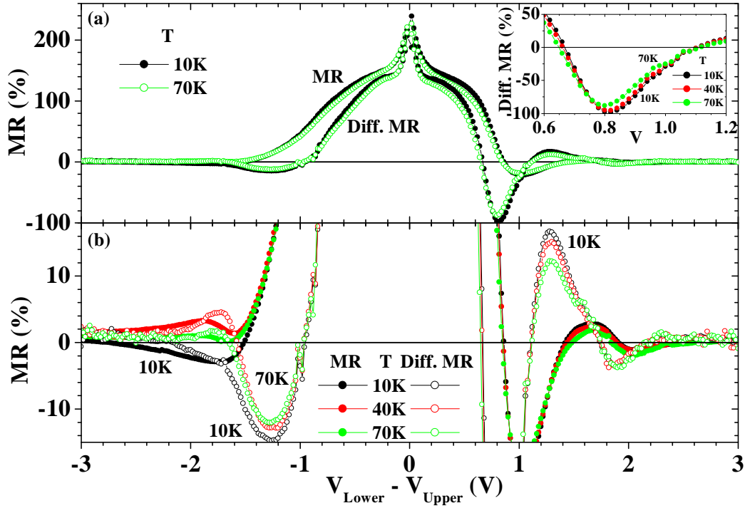
Figure 7.15: LSMO/STO/LSMO, Junction C in V_{Desc} = +3\text{V} state: (a) bias dependence of TMR and differential TMR at T = 10\text{K} and 70\text{K} . The inset to panel (a), and panel (b), are closeups of panel (a) for T = 10\text{K} , 40\text{K} and 70\text{K} .
