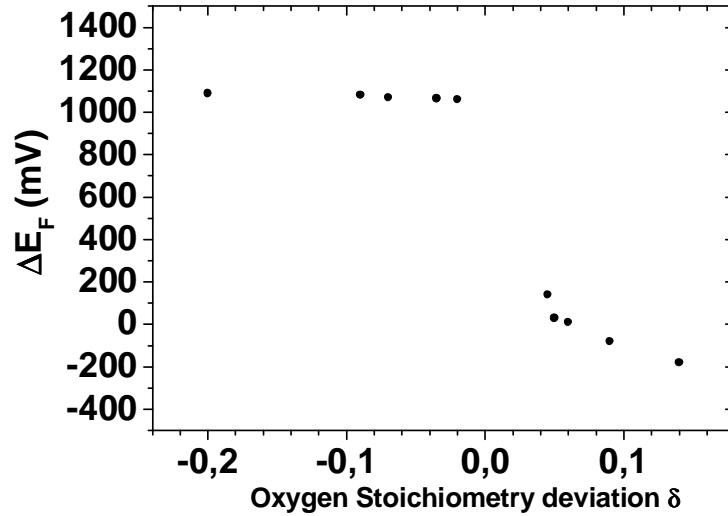
Figure A.16: Evolution of the Fermi level of La_{0.9}Sr_{0.1}MnO_{3\pm\delta} at 873K with oxygen concentration. Adapted from Ref. [184]
