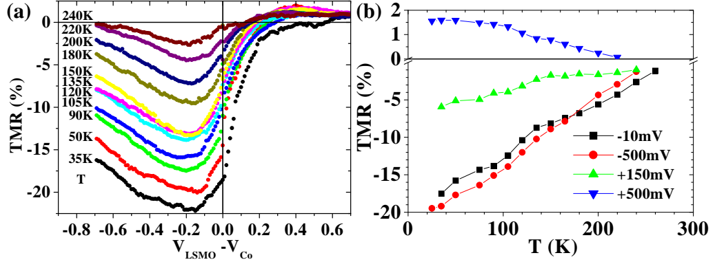
Figure 6.4: Bias and temperature-dependent TMR response of a LSMO/STO/Co junction ( \text{Al}_{15}\text{S}_{11}\text{A}=80\mu\text{m}^2 ): (a) evolution of the TMR bias dependence with temperature and (b) temperature evolution of TMR at remarkable bias values.
