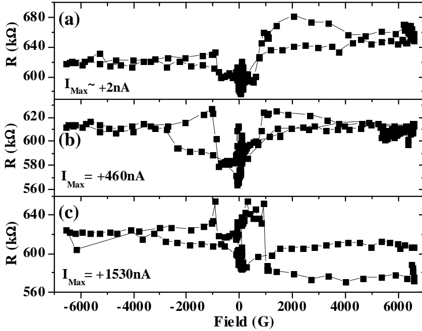
Figure 7.6: Sample C: LSMO/STO/Co 80 Cr 20 junction of area 12 \mu\text{m}^2 . First R(H) loops of a at T=4K and V=+1mV, with a history of injected current I_{Max} = (a) +2nA, (b) +460nA and (c) +1530nA.
