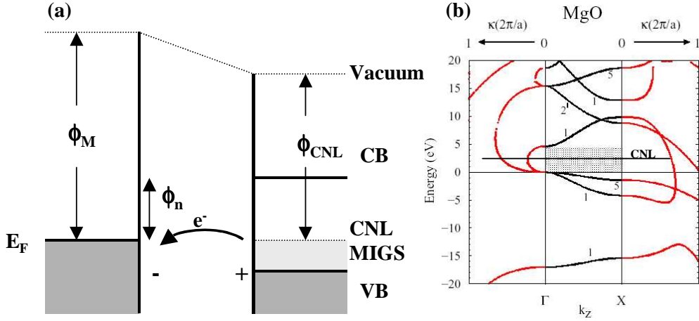
Figure 2.5: (a) Schematic band structure of MIGS at a Metal/Semiconductor interface. (b) Complex band structure of \text{MgO}(001) by Bellini [41]
