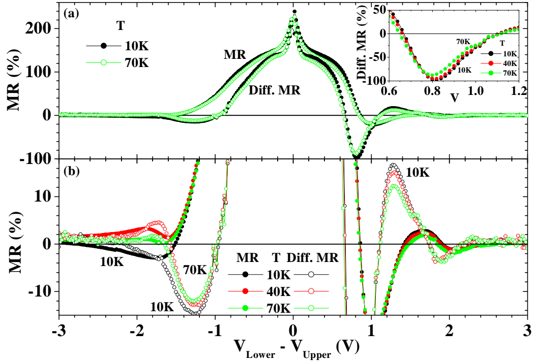
Figure 7.15: LSMO/STO/LSMO, Junction C in V_{Desc} = +3V state: (a) bias dependence of TMR and differential TMR at T=10K and 70K . The inset to panel (a), and panel (b), are closeups of panel (a) for T=10K , 40K and 70K .
