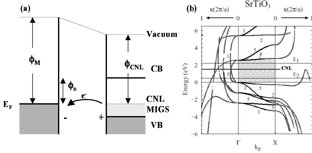
Figure A.8: (a) Schematic band structure of MIGS at a Metal/Semiconductor interface. (b) Complex band structure of \text{SrTiO}_3 (001) by Bellini [41]
