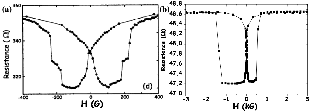
Figure 4.2: LSMO/I/Co: R(H) loops at V=10\text{mV} for (a) I=\text{Ce}_{0.69}\text{La}_{0.31}\text{O}_{1.845} and (b) I=\text{TiO}_2 . The asymmetric loop found in the case of TiO 2 reflects AF pinning by CoO atop the Co layer.
