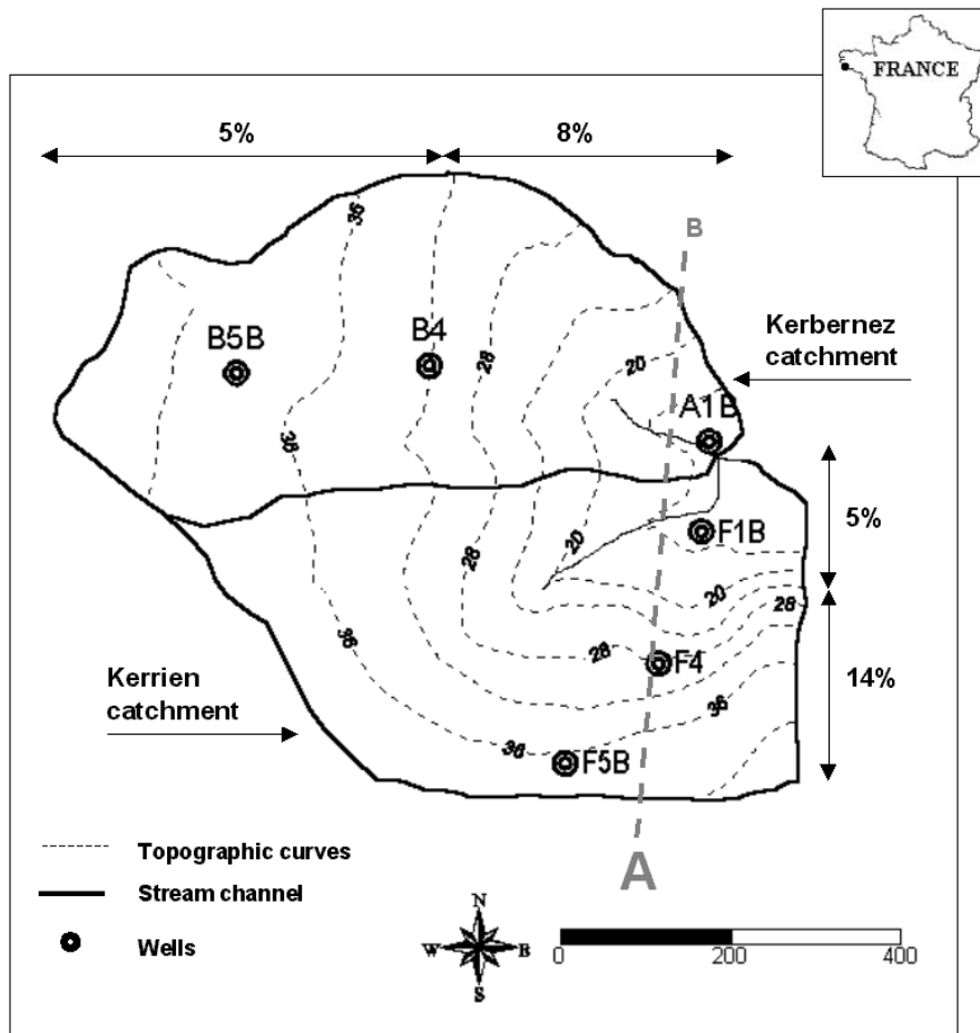
FIG. 4.6 – Study site location, wells positions and surface slopes along the hillslopes of Kerbernez and Kerrien catchments.
