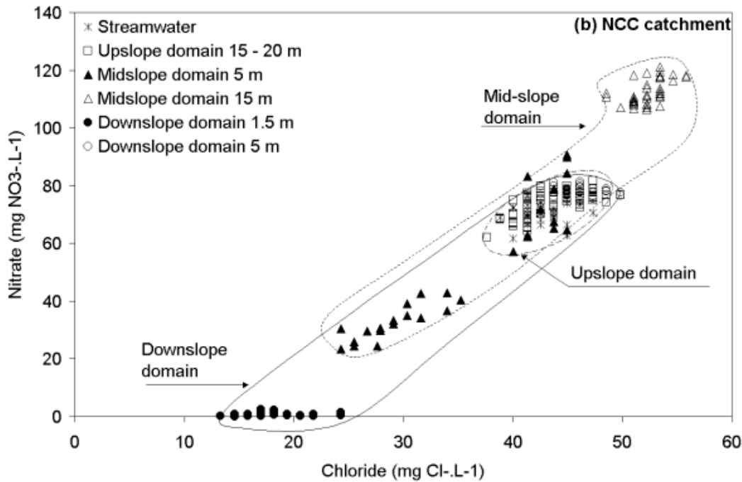
FIG. 3.16 – Nitrate and chloride concentrations during the whole period in the different domains of the CC catchment (a) and NCC catchment (b). For the sake of clarity, only specified wells (underlined on table 1) have been chosen to represent domains.
