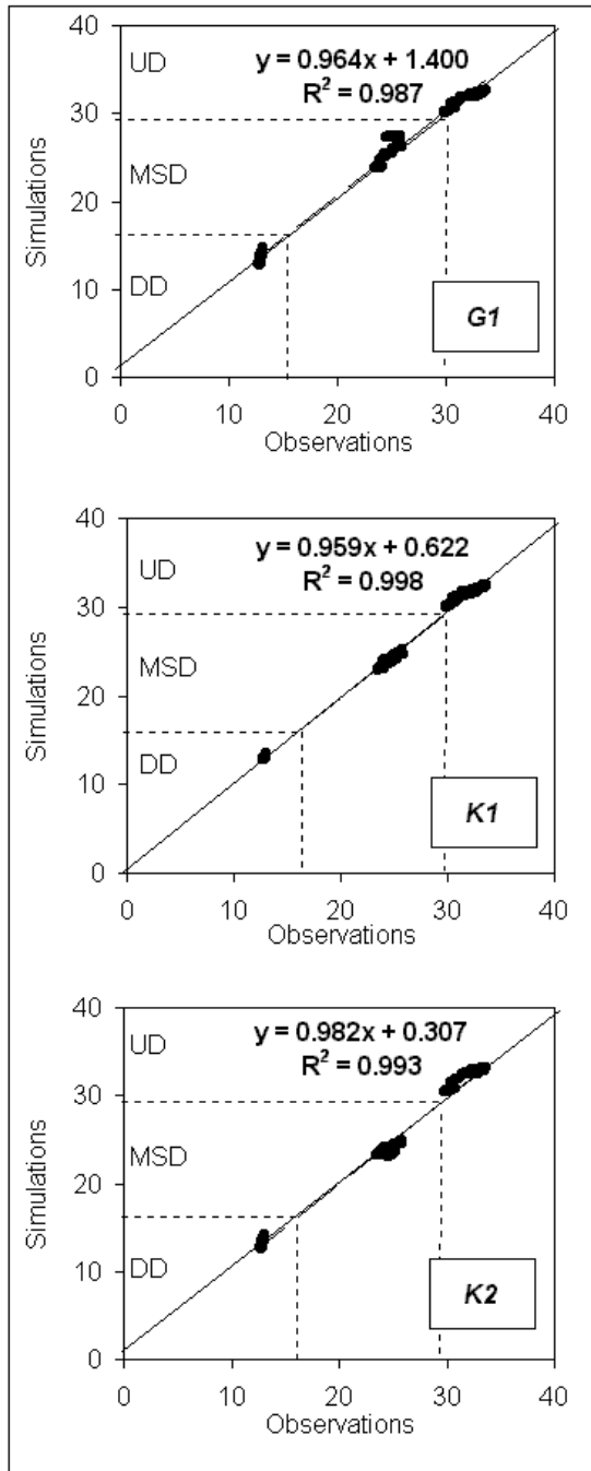
FIG. 4.11 – Observed and simulated water table elevations (m above sea level) with G1, K1 and K2 flow domains during the calibration period for the Kerbernez and Kerrien catchments. Downslope domains (DD), midslope domains (MSD) and upslope domains (UD) are separated by dashed lines. Black line represents the 1 :1 line. Coefficients of correlation ( R^2 ) and the best linear regression between observations and simulations are also indicated.
