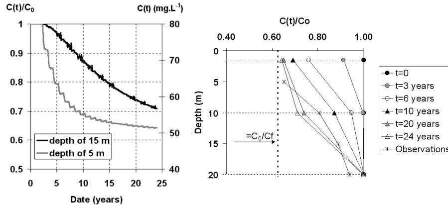
FIG. 4.17 – Evolution of groundwater nitrate concentrations following a decrease of recharge concentrations. C_0 ( 80 \text{ mg.L}^{-1} ) and C_f ( 50 \text{ mg.L}^{-1} ) are initial and final nitrate concentration in the water recharge, respectively. The 20 m depth corresponds to the WGA-bedrock interface.
