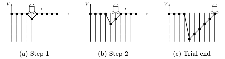
Figure 3.3: Monte-Carlo method (TD(1))
