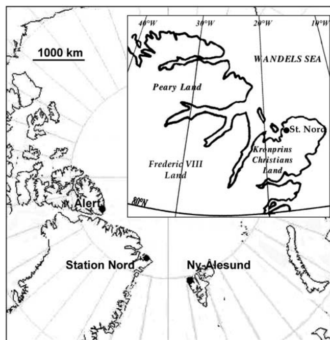
Fig. 2 Location of Station Nord in northern part of Greenland
