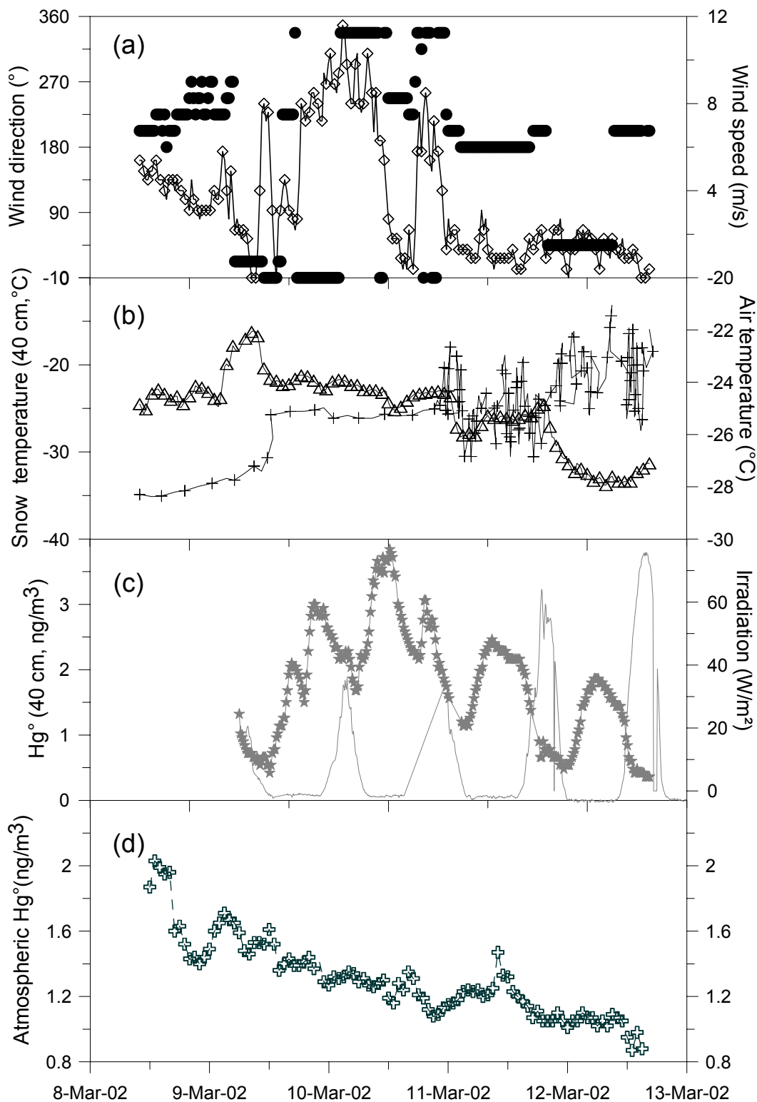
Figure IV.10 Continuous monitoring of (a) wind direction (●) and wind speed (◇), of (b) atmospheric temperature (△) and snow temperature at 40 cm below the snow surface (+), of (c) Hg° concentrations in snow air at 40 cm depth (★) and solar irradiation above the snow (—) and of (d) ambient Hg° concentration (⊕) in Station Nord from March 9 h to March 13 h , 2002.
