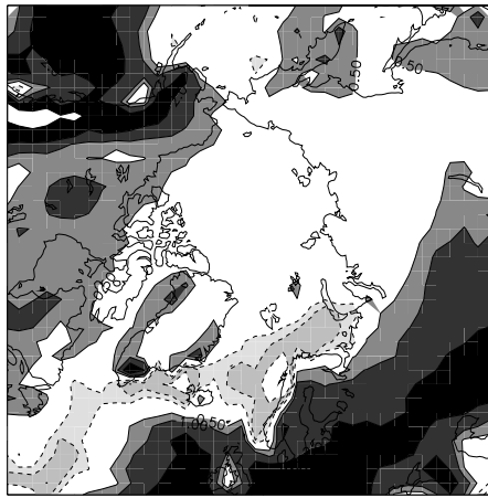
PD-NF - L&W (winter)
