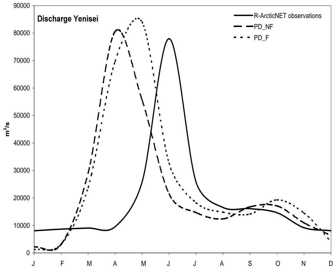
Fig. 2.21 : Monthly Yenisei river discharge ( \text{m}^3/\text{s} ) as measured at the station Igarka ( 67.43^\circ\text{N} ; 86.48^\circ\text{E} ) over the period 1985-1995 [ Lammers et al. (2000) ] and estimated in PD-NF and PF-F experiments.
