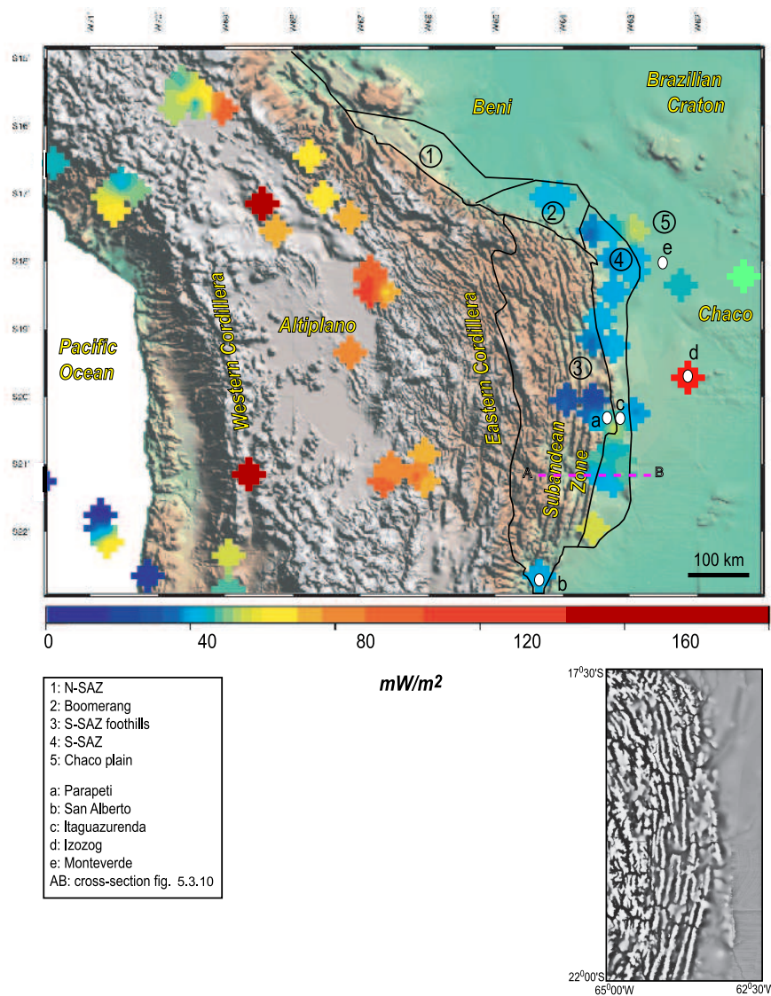
FIG. 2.1.2 – Thermal data (diamonds) in the Andes between 15^{\circ}S and 23^{\circ}S (modified after Sclater et al., 1970, Uyeda and Watanabe, 1982, Henry and Pollack, 1988, and Springer and Förster 1998) overlain on a digital elevation map. Box : periodic setting evidenced by filtering of topographical high frequencies. Solid black lines are the limits between the domains numbered from 1 to 5.
