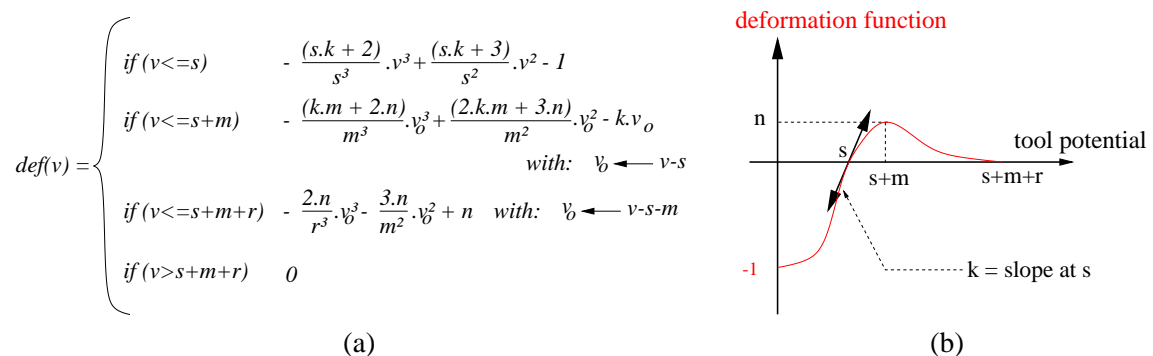
FIG. 2.9: Deformation function : (a) equation et (b) parameters.
