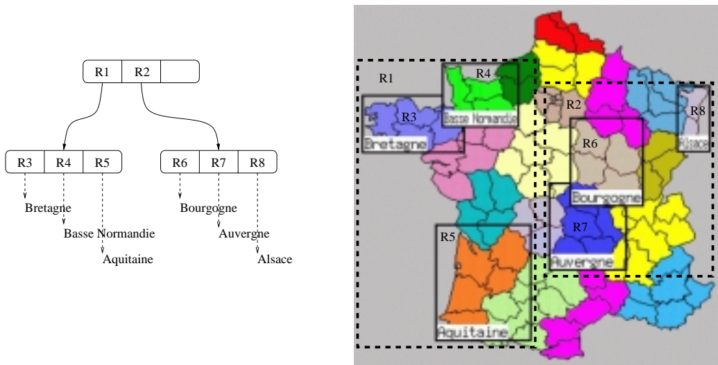
FIG. 2.2 – Structure R-tree
