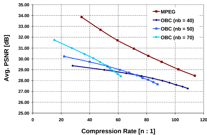
FIG. 8.2: BILLS2 sequence : Avg. PSNR in [dB] vs. Compression Rate in n : 1 for MPEG and OBC encoding in various configurations. nb indicates the number of basis images used.
