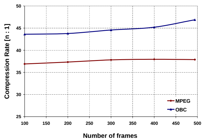
FIG. 8.13: CLAIRE sequence : Compression Rate in n : 1 versus number of frames for MPEG and OBC encoding.
