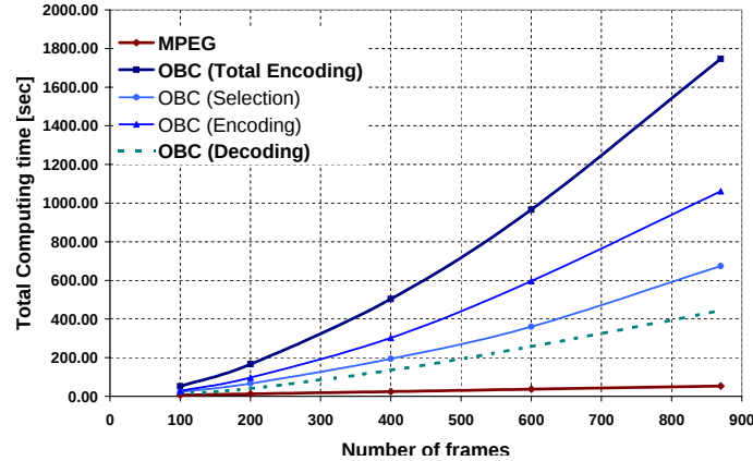
FIG. 8.29: Sequence GRANDMA : Computing time in [sec] vs. number of frames to be encoded. The basis size is adapted to yield an approximatively constant reconstruction quality.
