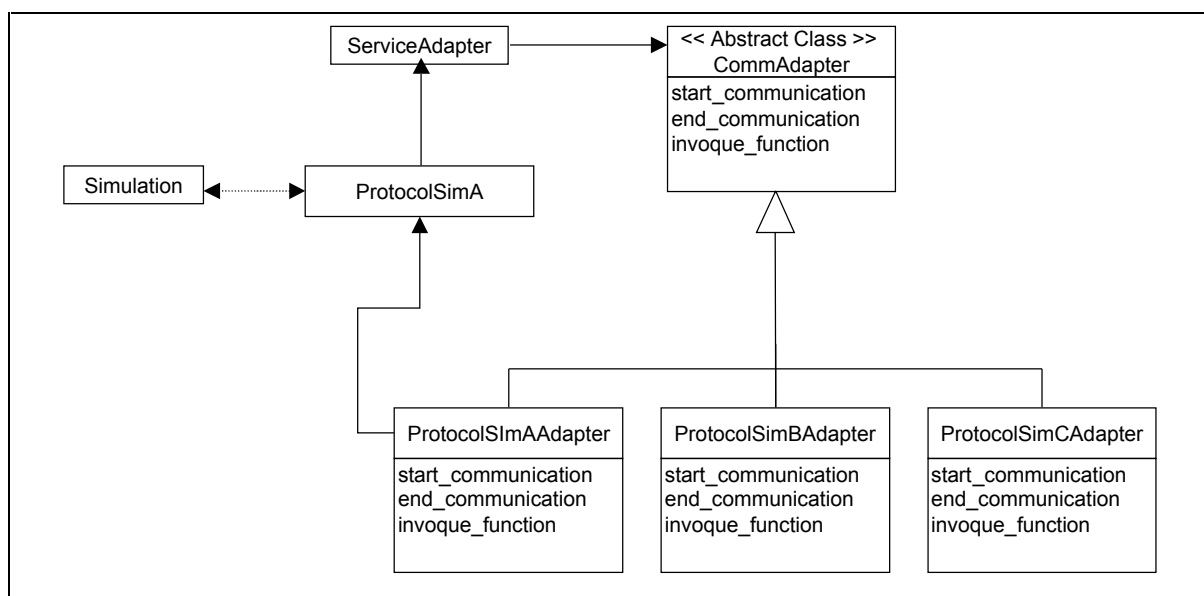
Figure 8-5: Schéma de classes du composant CommAdapter d'ARGOS
