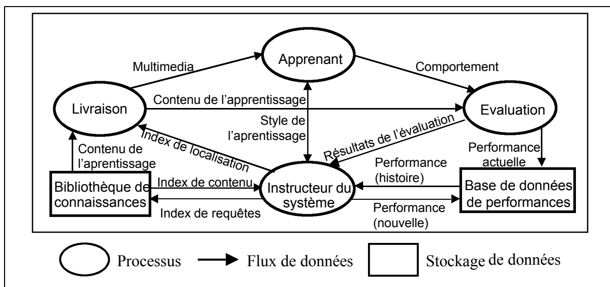
Figure 7-1: Composants de l'architecture LTSA
