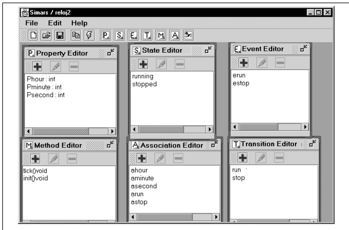
Figure 6-12: Interface du prototype de SIMARS
