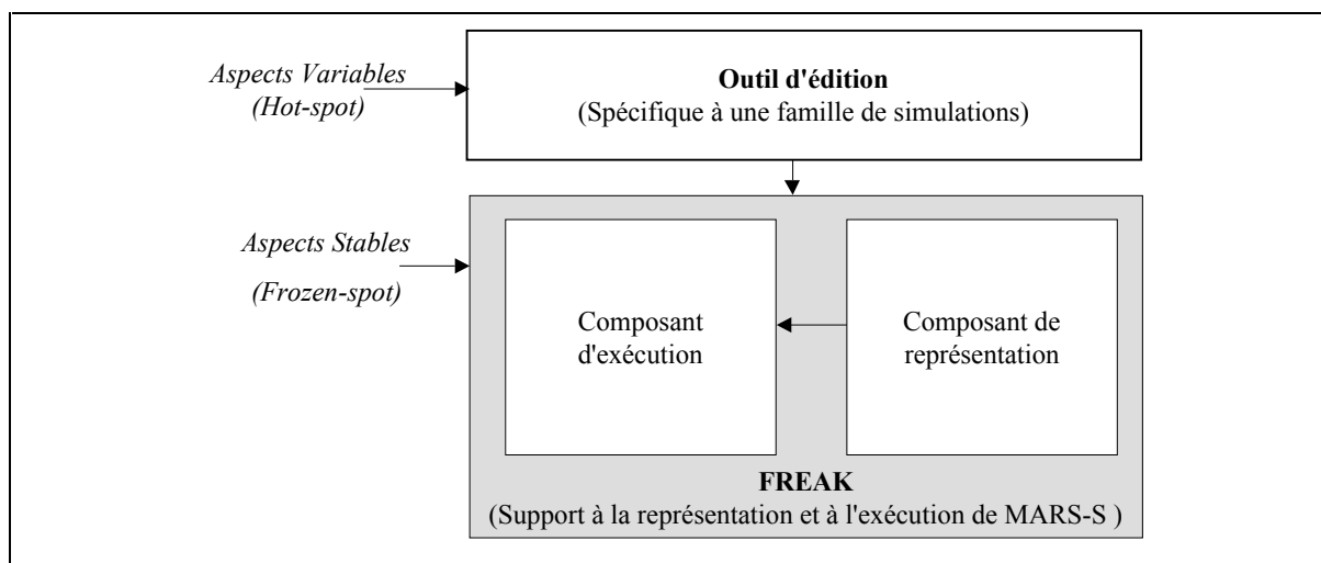
Figure 6-5: Structure globale du framework
