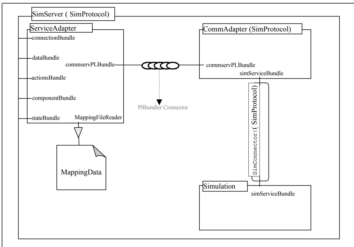
Figure 8-4: Description graphique du composant SimServer
