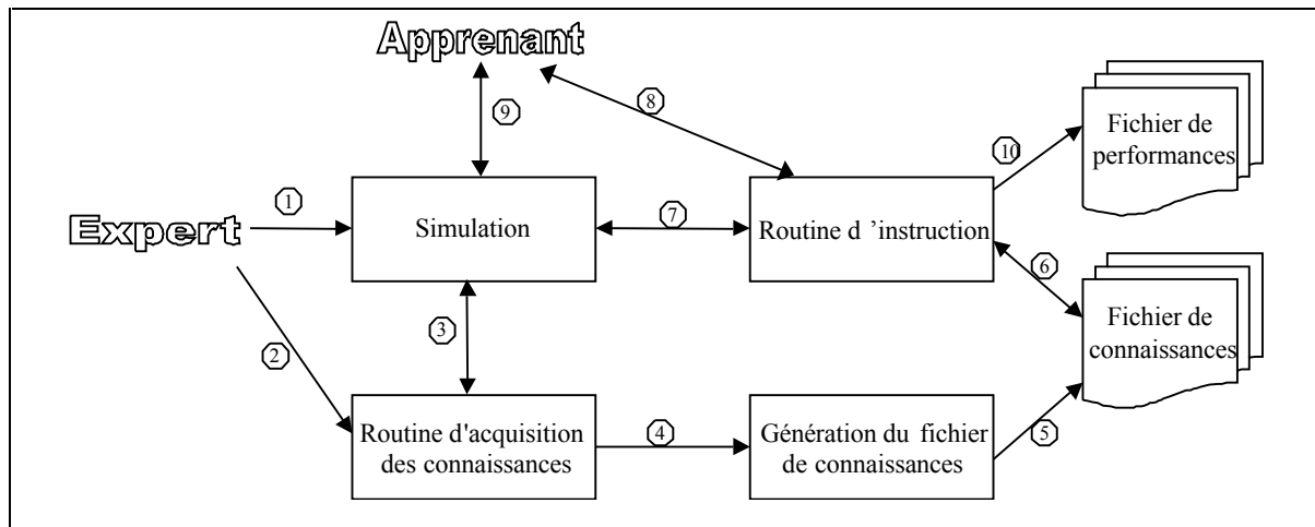
Figure 3-7: Le processus CGT
