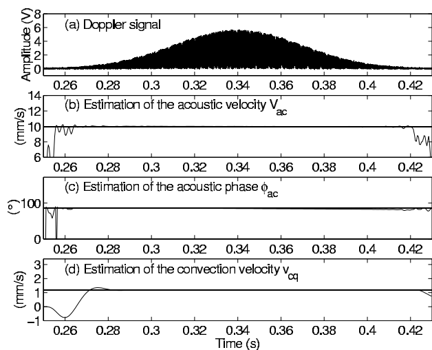
Fig. 4. Estimation of amplitude (b), phase (c) and convection velocity (d) of the acoustic velocity.
