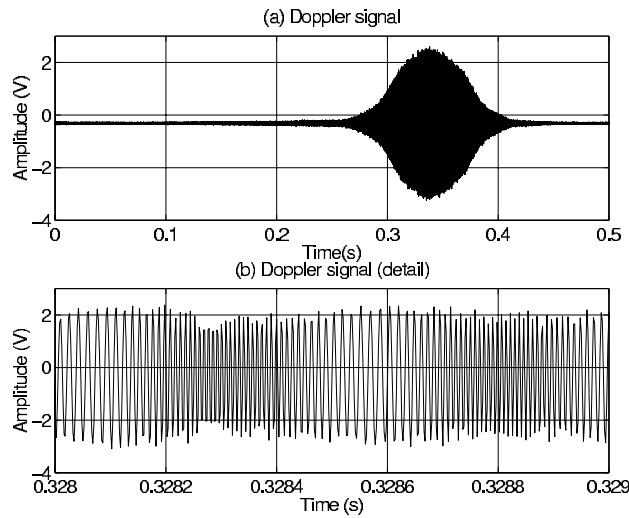
Fig. 2. Time representation of an experimental Doppler signal (a) and detail (b) showing the frequency modulation ( F_{ac} = 1000 Hz, V_{ac,eff} = 20 mm/s).
