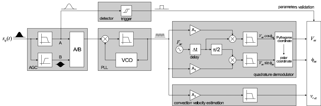
Fig. 3. Block diagram of the acoustic parameters estimation technique.
