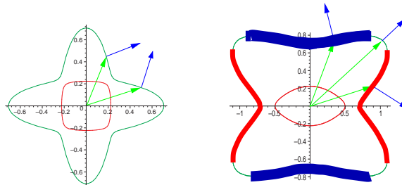
FIG. 3.2: Slowness diagrams. Left: material (II) - Right: material (III).
