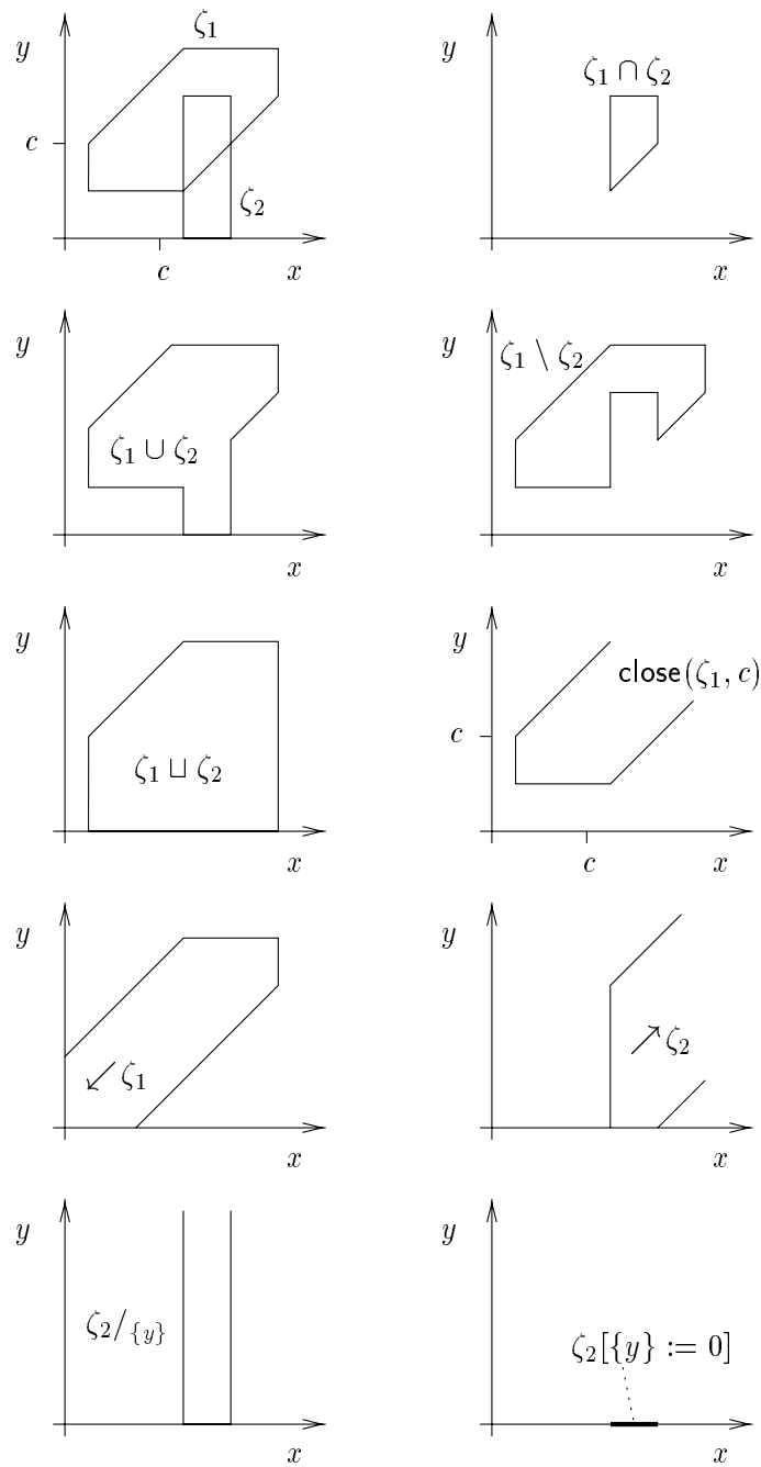
Figure 2.3: Polyhedra on \{x, y\} and their operations.
