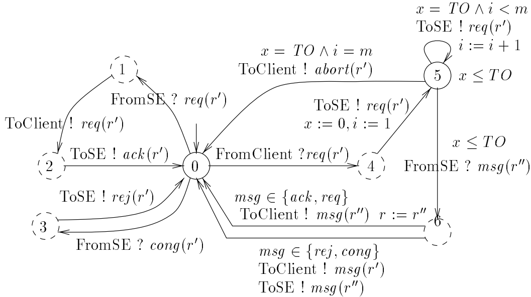
Figure 12.20: The left FRPU of the FRP-DT example.
