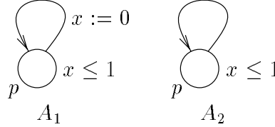
Figure 5.9: Time-abtracting bisimulations do not preserve non-zenoness.
