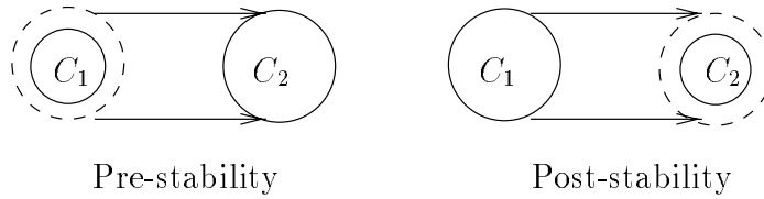
Figure 2.1: Pre- and post-stability.
