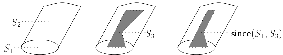
Figure 7.10: Illustration of the \text{etctl-post}() operator.
