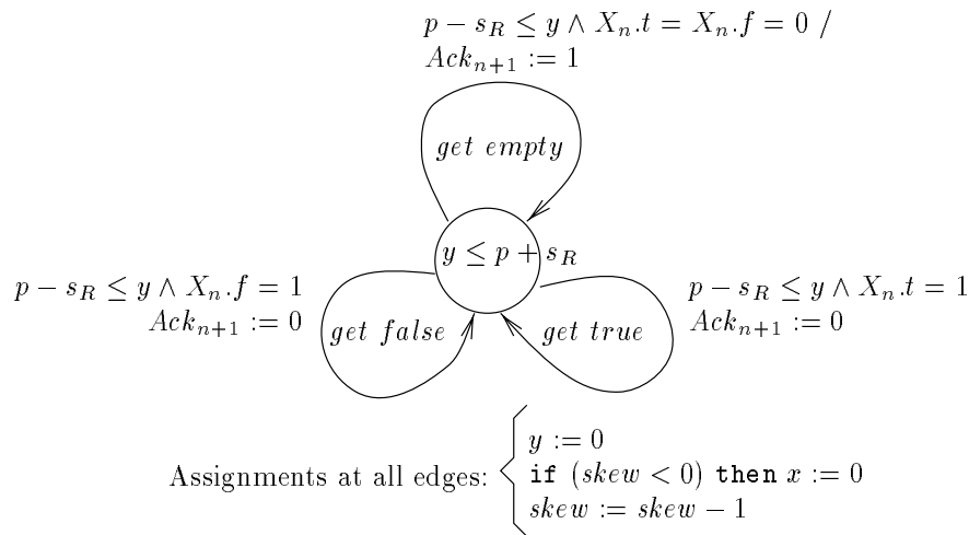
Figure 12.11: The receiver.
