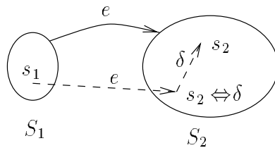
Figure 5.13: Post-stability in the simulation graph.
