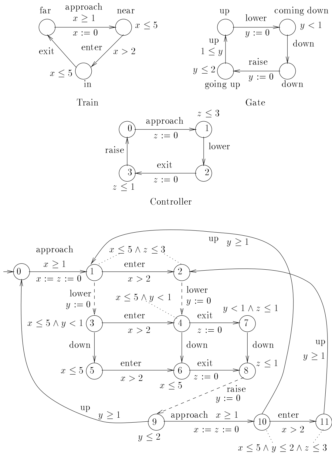
Figure 9.2: The composite CTA for the TGC system.
