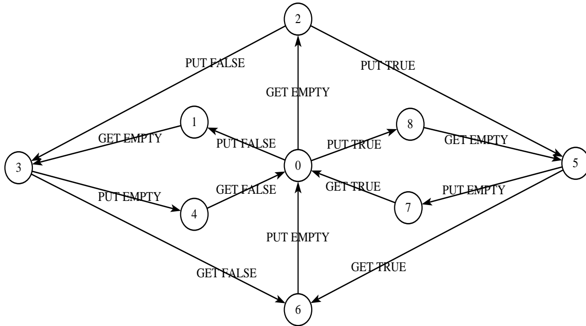
Figure 12.12: 3-stage Stari.
