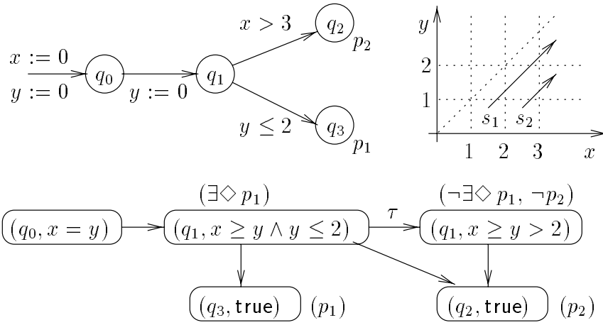
Figure 5.11: Weak time-abtracting bisimulations do not preserve CTL.
