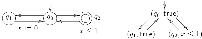
Figure 7.8: Elementary cycles do not suffice for non-trivial acceptance conditions.
