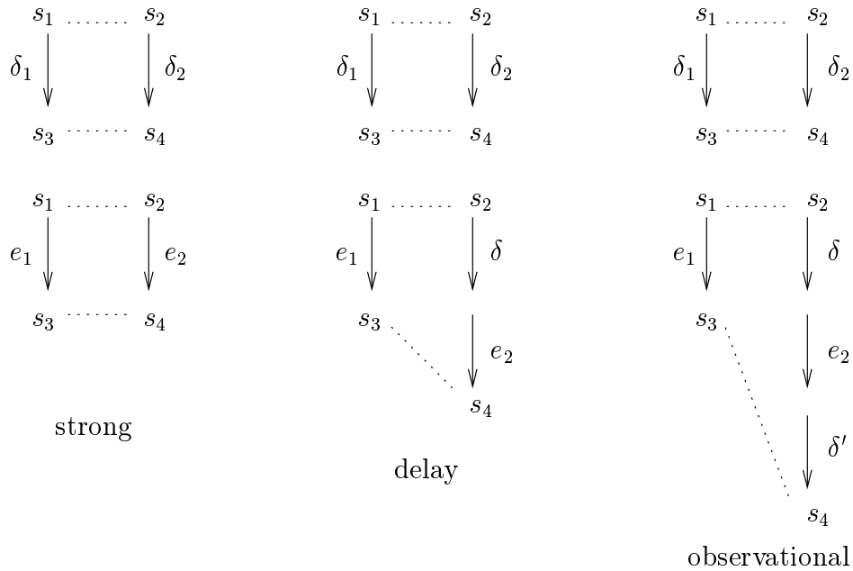
Figure 5.2: Time-abtracting bisimulations.
