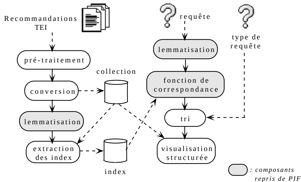
Figure 5.1. Architecture générale du prototype
