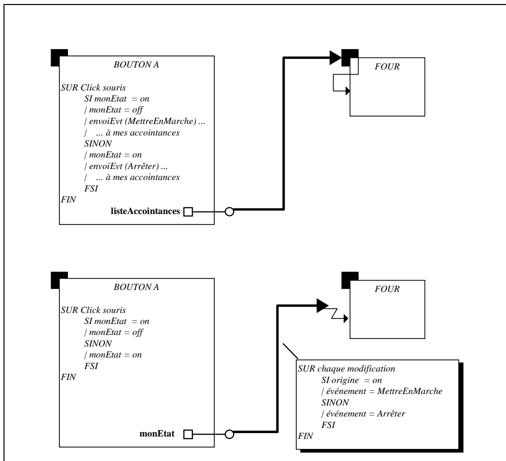
Figure 10-10 : Association simple et Association intelligente
