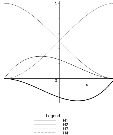
FIG. 3.2: The Hermitian finite elements .
