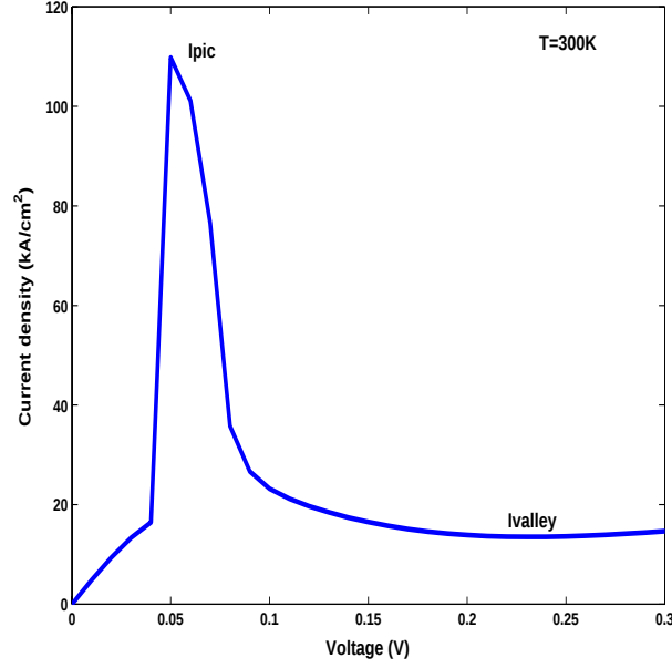
FIG. 5.5: The current-voltage for an InAs/AlSb/GaSb/AlSb/InAs resonant interband tunneling with 10Å AlSb barriers and 30Å GaSb well when P = 1.4 \times 10^6 \text{ eV}\cdot\text{m} .
