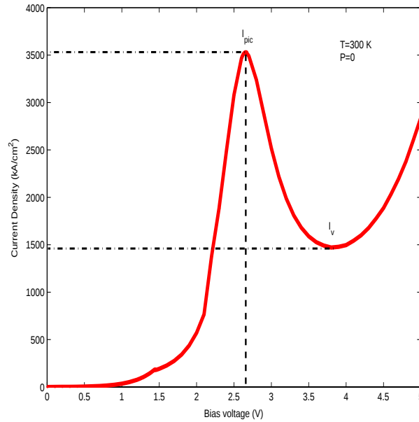
FIG. 5.4: The current-voltage for an InAs/AlSb/GaSb/AlSb/InAs resonant interband tunneling with 10Ang AlSb barriers and 30Ang GaSb well when P = 0 .
