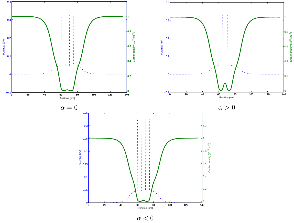
FIG. 3.8: The charge density in 10^{18} \text{cm}^{-3} and the potential at a bias of V = 0 Volt for both parabolic ( \alpha = 0 ) and non-parabolic ( \alpha > 0 and \alpha < 0 ) energies.
