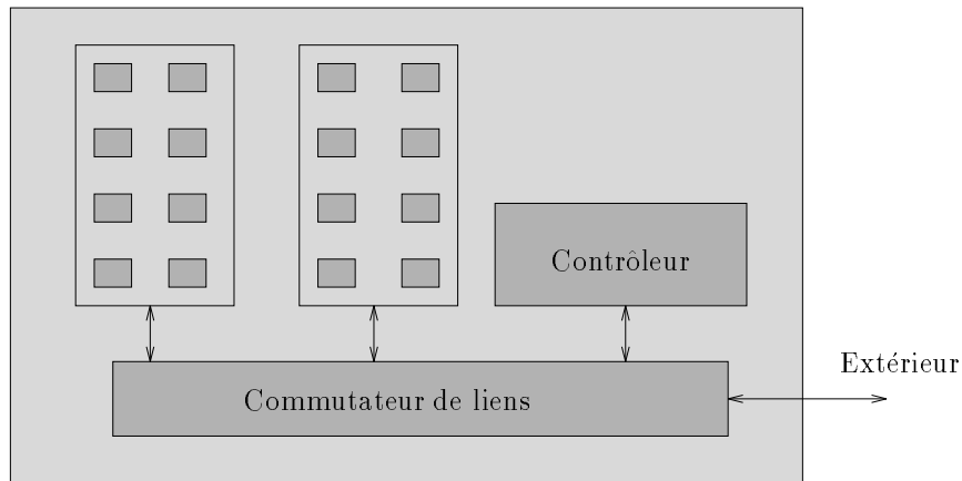
Figure 4.1: La machine Tnode à 16 Transputers.
